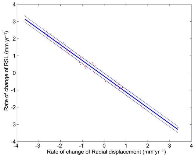
Fig. 4 Relationship between predicted vertical uplift rate and rate of RSL change for the ICE-5G (VM2) model, version 1.3 (Peltier, 2004) and ICE-6G (Peltier et al., 2015) indicated by red dots. The solid blue line is the regression: \langle \text{Rate of relative sea-level change} \rangle = -0.9167 \times \langle \text{vertical uplift} \rangle - 0.1947 . The dashed lines mark the range of two standard deviations of the error.
