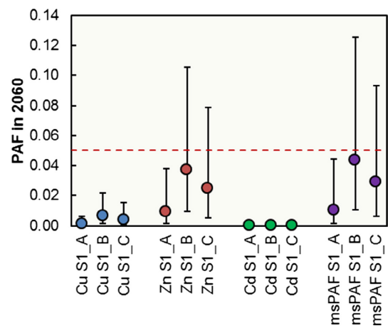
Fig. 11. Predicted PAFs for Cu, Zn, Cd, and msPAFs, for under historic input scenario S1 and future input scenarios A, B, and C, in 2060. Points are the msPAF 50 s, error bars are ±1 SD. The horizontal dashed line represents the msPAF above which potential risks to the ecosystem are conventionally considered to be indicated.
