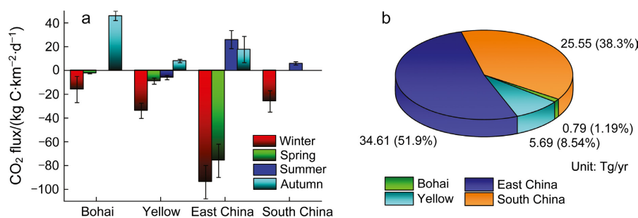
Fig. 3. Seasonal changes in CO 2 fluxes in the air–sea interface. The part below zero means a C sink, and the part above zero means a C release (a); the annual net CO 2 uptakes or releases by the China Seas (b).
