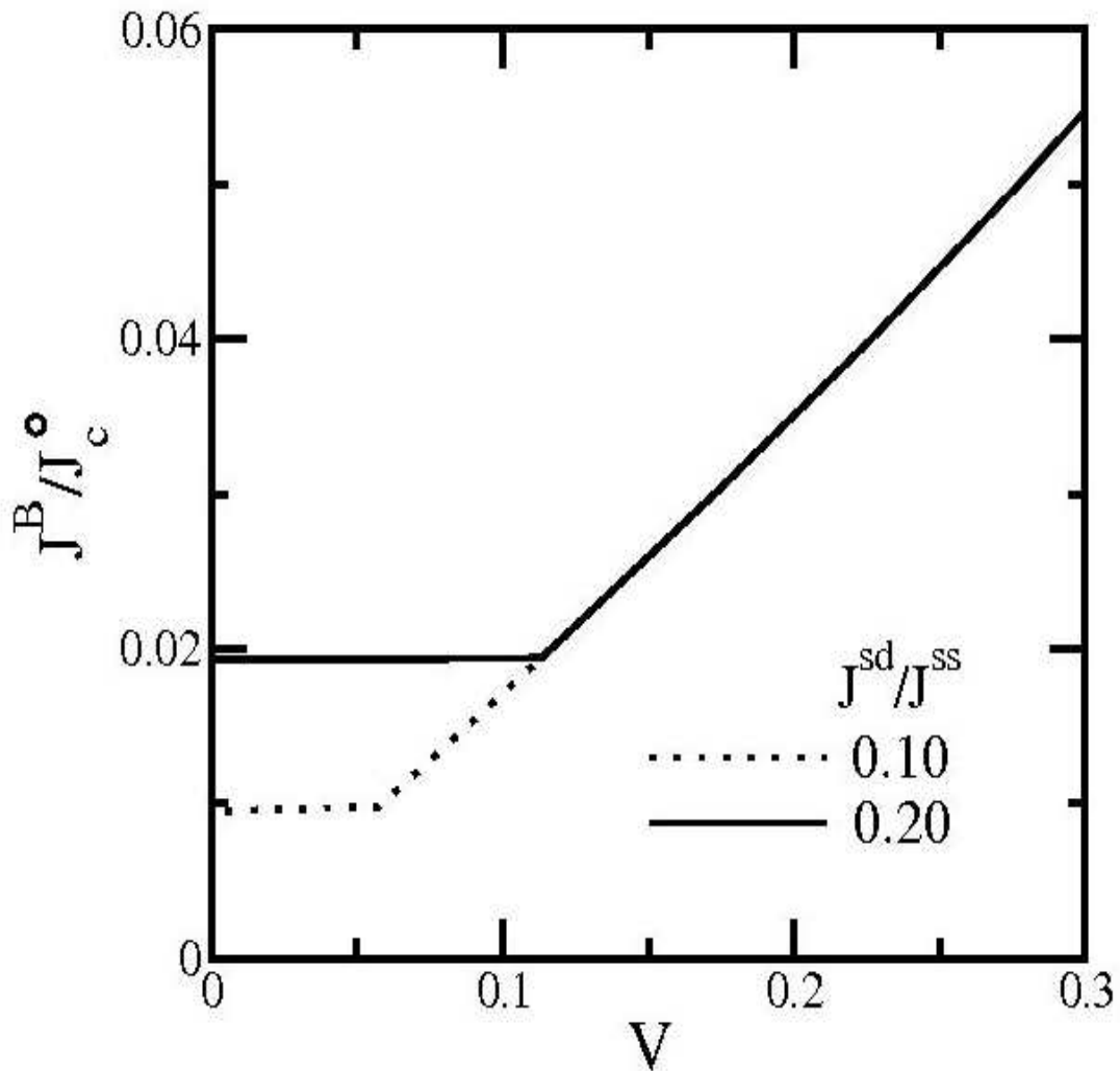
Figure 17. The current-voltage curves for J^{sd}/J^{ss}= 0.1 (dotted line) and J^{sd}/J^{ss} =0.2 (solid line) illustrate the dependence of the threshold bias current on the Josephson current. Here, the dissipation parameters are \Gamma_1 = 0.1 , and \Gamma_2= 0.1 .
