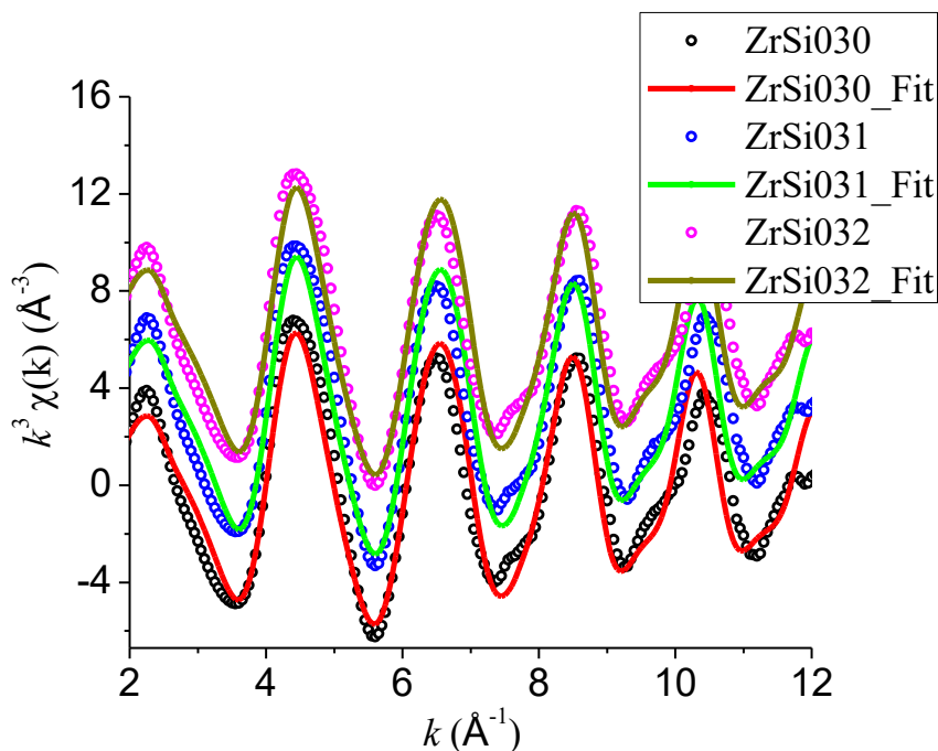
Figure 60. Experimental (dotted line) EXAFS functions k^3 \chi(k) ( \text{\AA}^{-3} ) and their best fits (solid line) of zirconium-doped lithium silicate samples ( p = 0.054 , s = 0.668 ) with different thermal treatments. The spectra and their fits are vertically separated by 3 \text{\AA}^{-3} for clarity.
