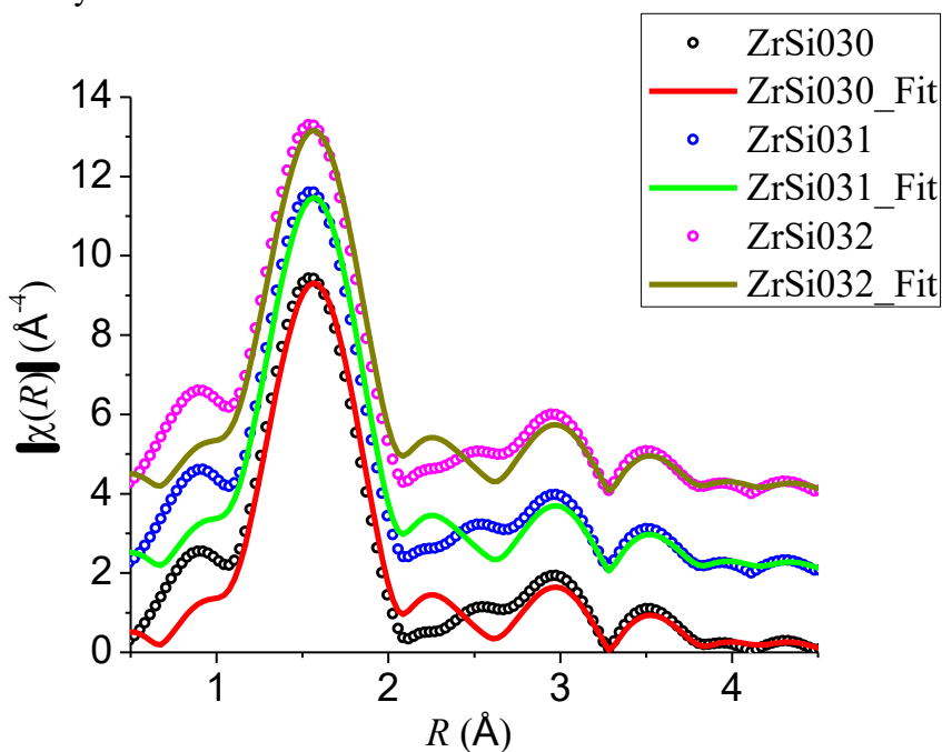
Figure 61. Fourier transforms of experimental (dotted lines) EXAFS functions in R -space and their fits (solid line) of zirconium-doped lithium silicate samples ( p = 0.054 , s = 0.668 ) with different thermal treatments. The spectra and their fits are vertically separated by 2 \text{\AA}^{-4} for clarity.
