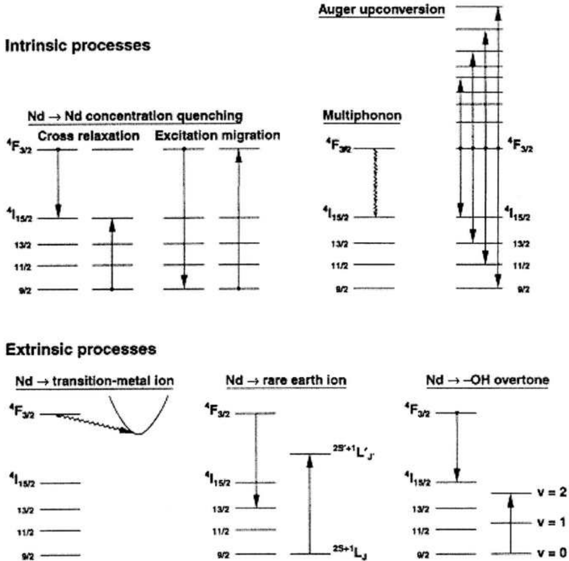
Figure 2. Non-radiative energy transitions between two nearby Nd 3+ cations (top), multiphonon interactions (top), and a Nd 3+ cation with others (bottom) [3].
