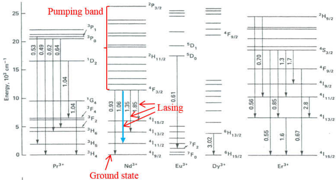
Figure 6. Radiative transitions of the five rare-earth ions studied. Wavelengths of transitions are in \mu\text{m} [6]. Typical four-level laser scheme is indicated for \text{Nd}^{3+} ion.
