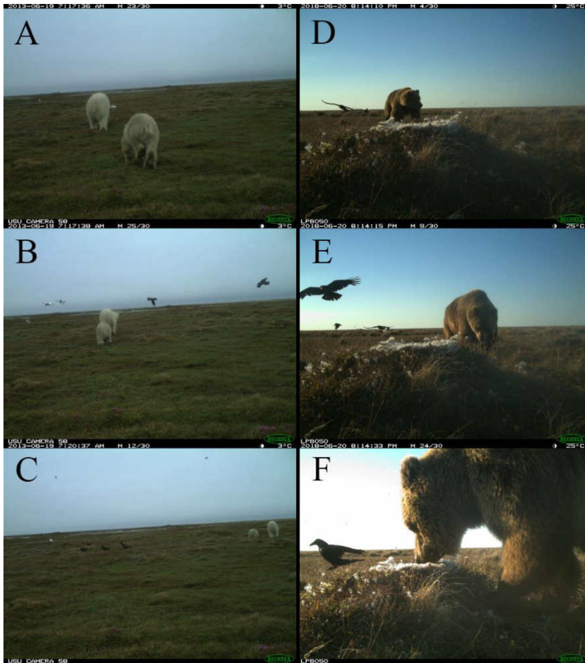
Figure 16 Observations of avian predators following bears foraging in a nesting snow goose colony. A-C) A female polar bear ( Ursus maritimus ) and cub cause a female lesser snow goose ( Anser caerulescens caerulescens ) to abandon its nest. Following predation of the nest, four common ravens ( Corvus corax ) inspect the nest for any unconsumed materials. D-F) A lone grizzly bear ( Ursus arctos ) approaches and consumes a lesser snow goose nest and is closely followed by at least three common ravens.
