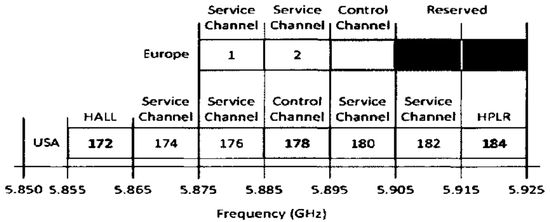
FIG. 15: DSRC overlapping channels in the EU and USA
