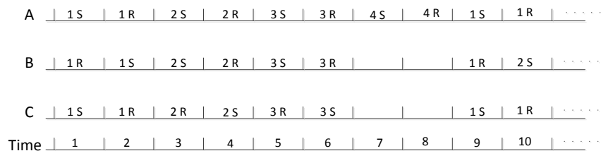
FIG. 47: Example Communication in DRIH-MAC. The nanonodes A , B and C from Figure 46 are shown. S indicates the sending mode, and R indicates receiving mode. The number preceding S/R indicates the color .
