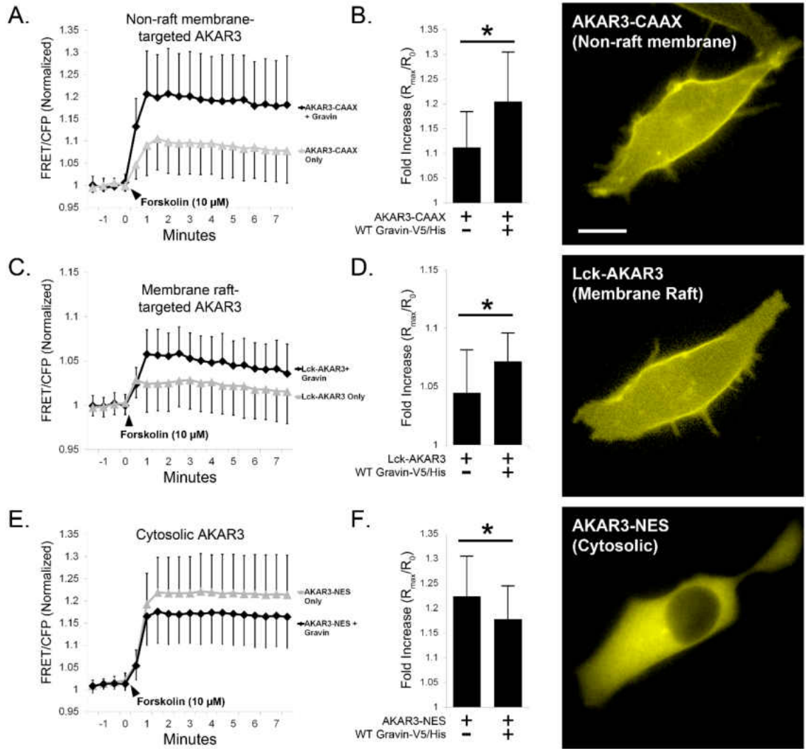
Figure IV-2. Gravin-V5/His expression alters subcellular PKA activity. AN3CA cells were co-transfected with gravin-V5/His and with AKAR3 constructs containing targeting sequences for non-raft membrane (CAAX), membrane raft (Lck), or cytosolic (NES) localization. Representative fluorescent images show the distribution the AKAR3 constructs. Expression of gravin increased forskolin-mediated PKA activity in both non-raft (A,B), and raft (C,D) membrane compartments. Conversely, gravin reduced PKA activity in the cytosol (E,F). Mann-Whitney Rank Sum tests revealed significant differences between the mean fold increases of each treatment. Asterisks denote p < 0.05 . Scale bar = 10 \mu m ; cells were incubated in 10 \mu M IBMX for 30 minutes prior to forskolin treatment.
