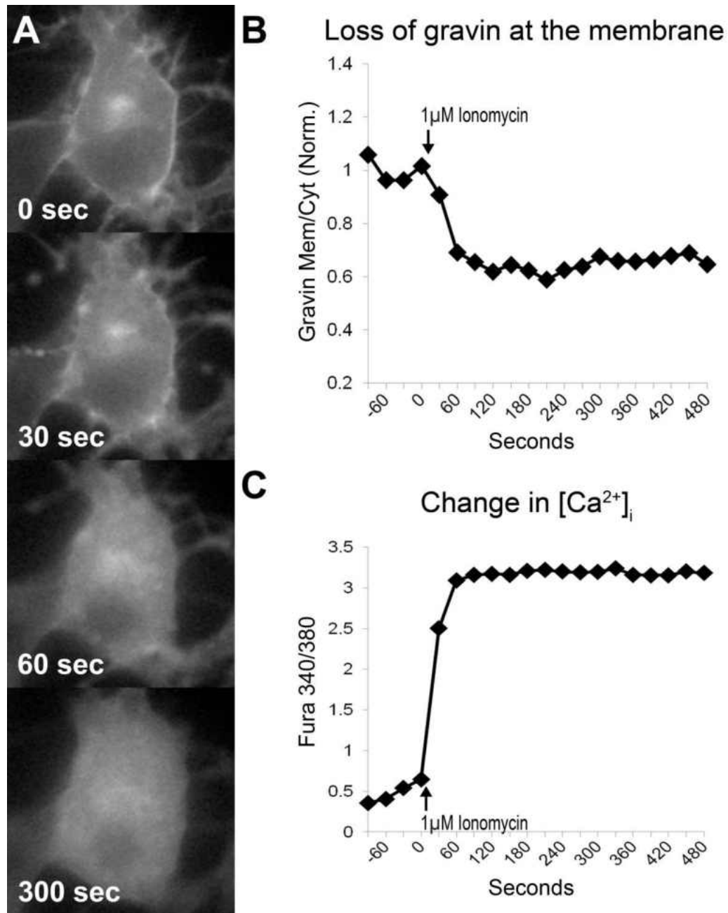
Figure III-1. Ionomycin treatment induces gravin redistribution. (A) Fluorescent micrographs illustrating that gravin-EGFP undergoes redistribution immediately following the addition of 1 \mu M ionomycin. (B) Plot of membrane:cytosol fluorescence intensity ratio over time illustrating the time course of gravin redistribution. (C) Corresponding plot of the Fura2 fluorescence ratio illustrating the rapid increase in [Ca^{2+}]_i upon ionomycin treatment. Note that gravin translocation is complete at t = 60 seconds, which corresponds to the time at which maximal cytosolic calcium increase is observed.
