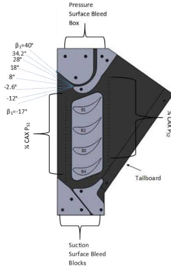
Figure 12: Modular cascade test section
