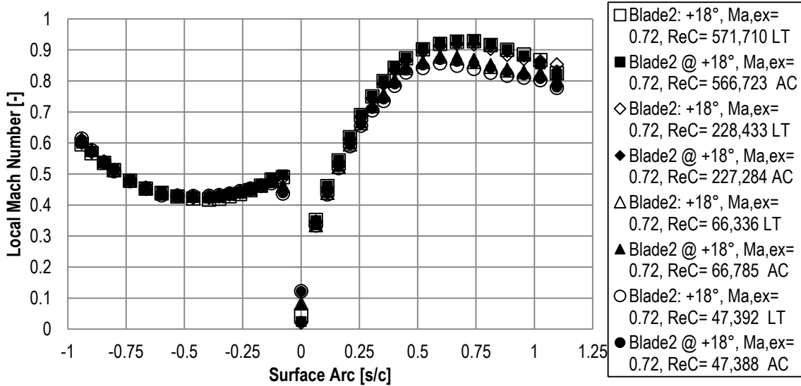
Figure 116: Midspan isentropic Mach distribution as a function of Reynolds number and turbulence intensity at 18° inlet angle.
