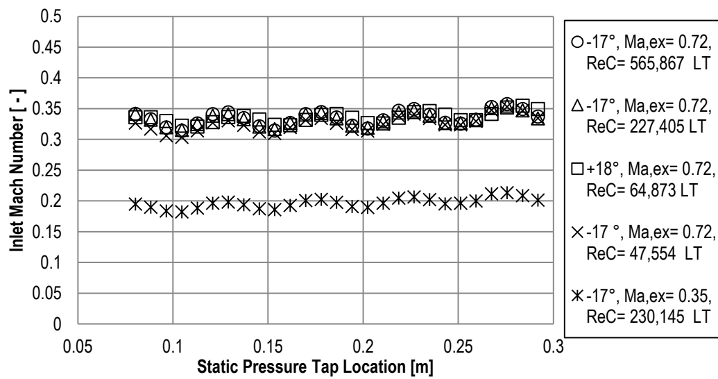
Figure 96: Inlet isentropic Mach distributions as a function of Reynolds number at -17^\circ inlet angle under low turbulence.
