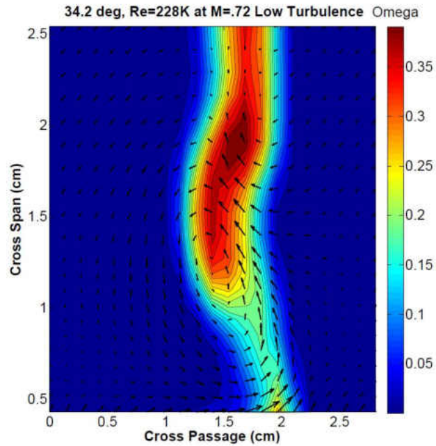
Figure 64: Contours of total pressure loss for Re_c = 227,500 at low turbulence and \beta_1 = 34.2^\circ
