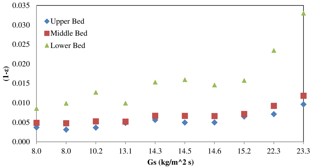
Figure 9. Solids Fractions in the Upper, Middle, and Lower Fast Bed locations for each recirculation rate observed at U_o \approx 3 m/s.
