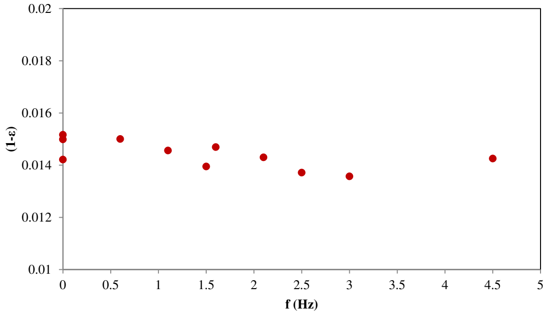
Figure 19. The Effect of Frequency On Solids Fractions for U_o \approx 2.8 m/s
