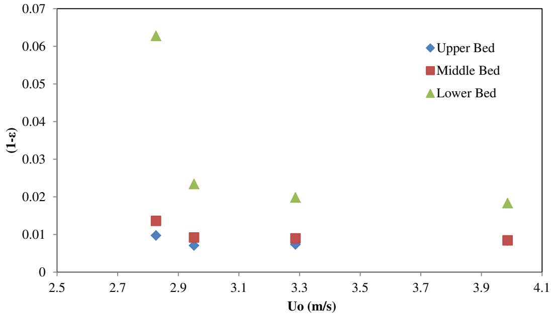
Figure 16. Variation of Solids Distribution At 3 Locations In the Fast Bed for G_s \approx 24 \text{ kg/m}^2 \text{ s} .
