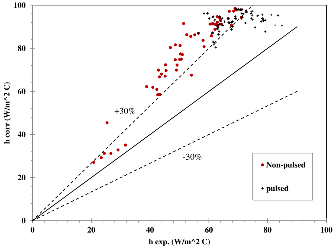
Figure 31. Parity Plot of Experimental Values vs. Eq. 5.5 Sundareshan and Kolar (2013)
