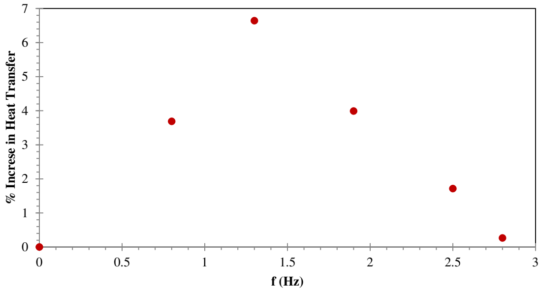
Figure 24. Percent Increase In Heat Transfer vs Frequency At 50% Valve Duty Cycle
