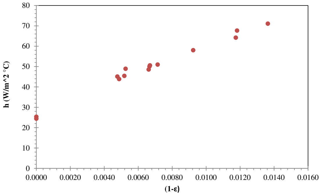
Figure 8. Solids Fraction vs. the Average Heat Transfer Coefficient for U_o \approx 3 \text{ m/s}
