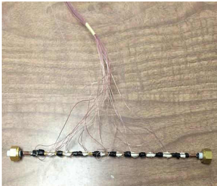
Figure 3.12 Square test section with thermocouples tips cemented axially along the surface using Omega bond cement.
