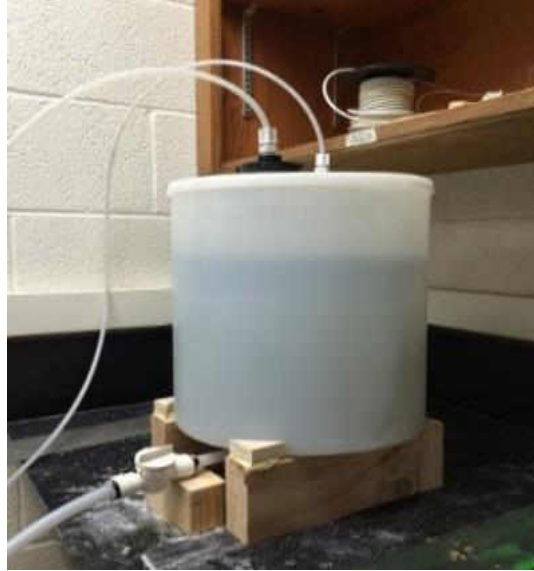
Figure 3.2 Flow loop reservoir.
