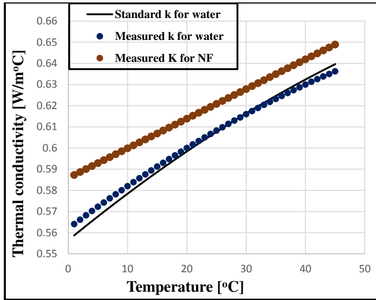
Figure 4.12 Comparison of the thermal conductivity vs. temperature for water and NF.
