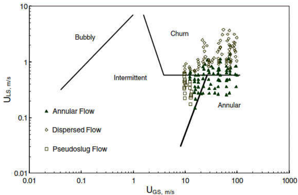
Figure 8. Pehlivan flow regime map compared to present experimental data [15]
