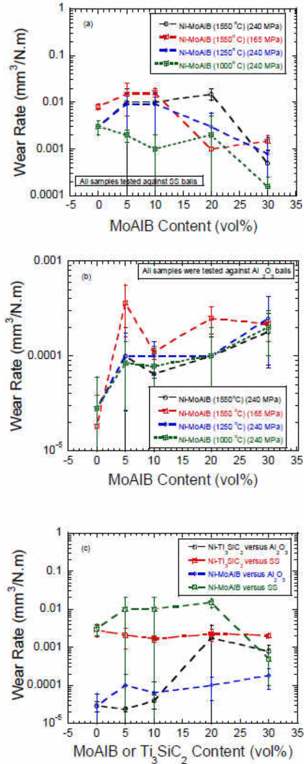
Figure 4.7: Plot of mean Wear Rate (WR) versus MoAIB content during sliding against, (a) SS, and (b) alumina balls, and (c) comparison of WR of Ni- \text{Ti}_3\text{SiC}_2 or Ni-MoAIB (1550 °C) after sliding against SS and \text{Al}_2\text{O}_3 balls, respectively.
