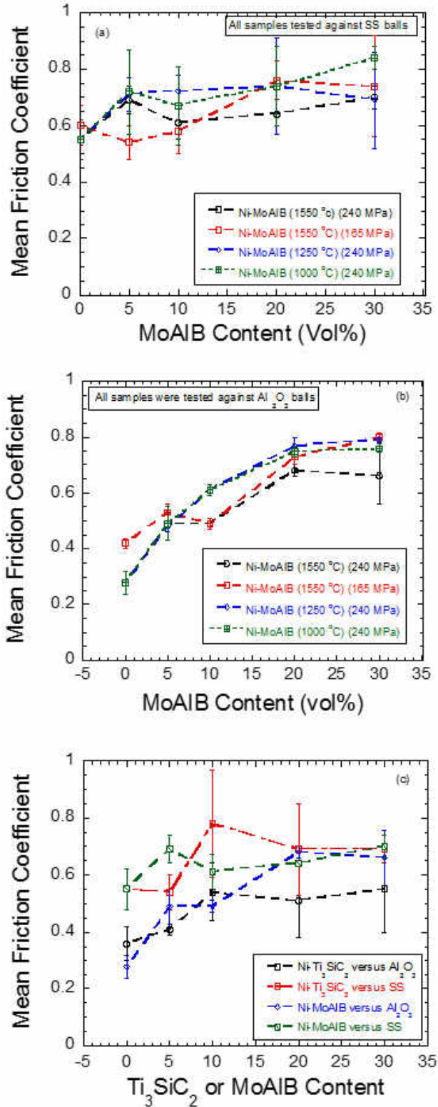
Figure 4.6: Plot of mean friction coefficient ( \mu_{\text{mean}} ) versus MoAIB content during sliding against, (a) SS, and (b) alumina balls, and (c) comparison of \mu_{\text{mean}} of Ni- \text{Ti}_3\text{SiC}_2 [13] or Ni-MoAIB (1550 °C) against SS and \text{Al}_2\text{O}_3 balls, respectively.
