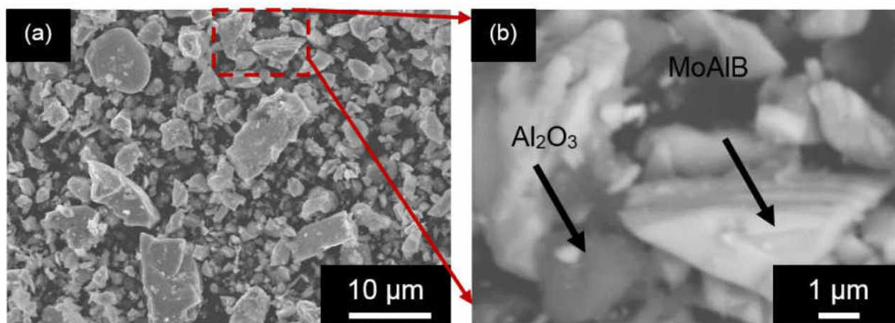
Figure 3.2: SEM SE micrograph of as-synthesized MoAlB particulates at, (a) lower, and (b) BSE image at higher magnifications.
