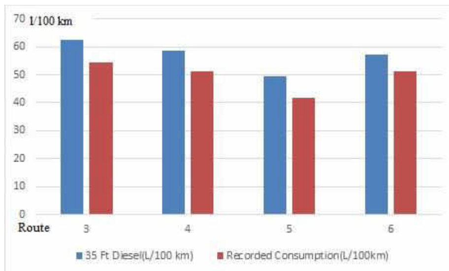
Figure 2.3 Model validation for 35 feet gasoline bus
