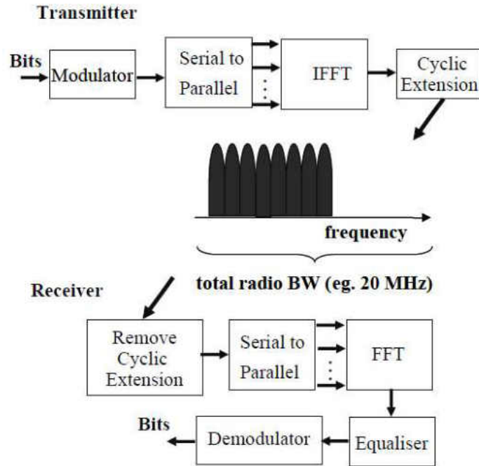
Figure 3: OFDMA transmitter and receiver [8]
