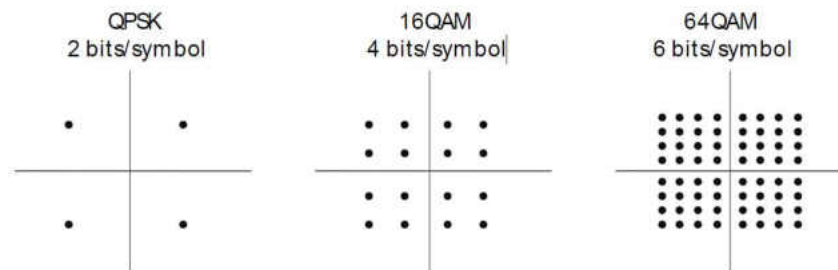
Figure 9: LTE Modulation Constellations [20]
