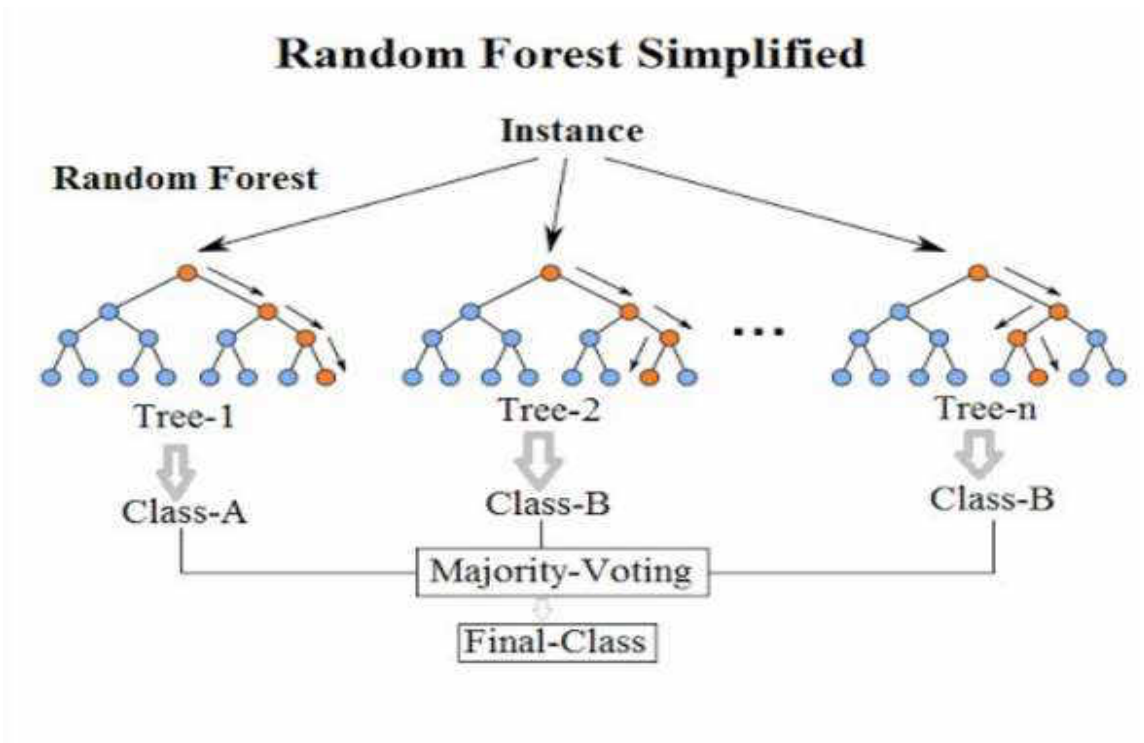
Figure 7: Random forest[26]
