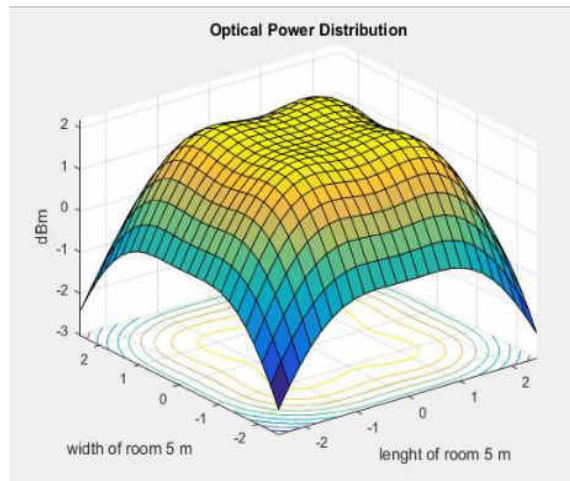
Figure 10. Optical power distribution in received optical plane for a FWHM of 70^\circ
