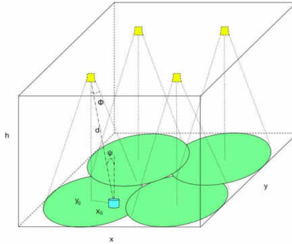
Figure 9. Representation of a room with four LEDs and their footprint [33].
