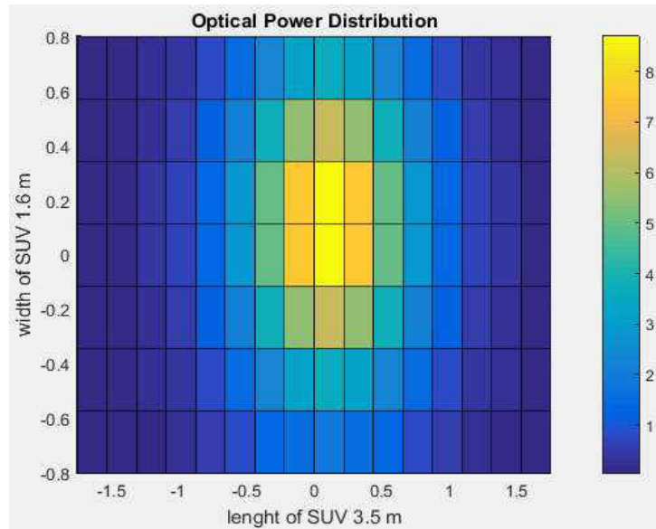
Figure 17. Optimized received power in mW for the rear and front passenger seats.
