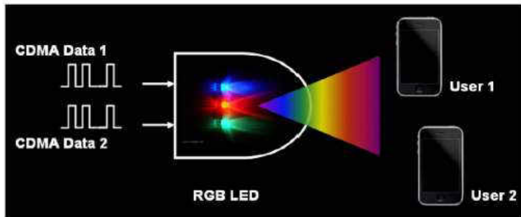
Figure 5. Proposed CSK-CDMA VLC system [16].
