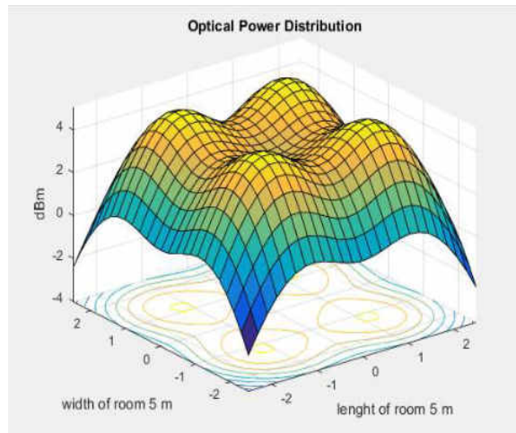
Figure 11. Optical power distribution in received optical plane for a FWHM of 35^\circ .
