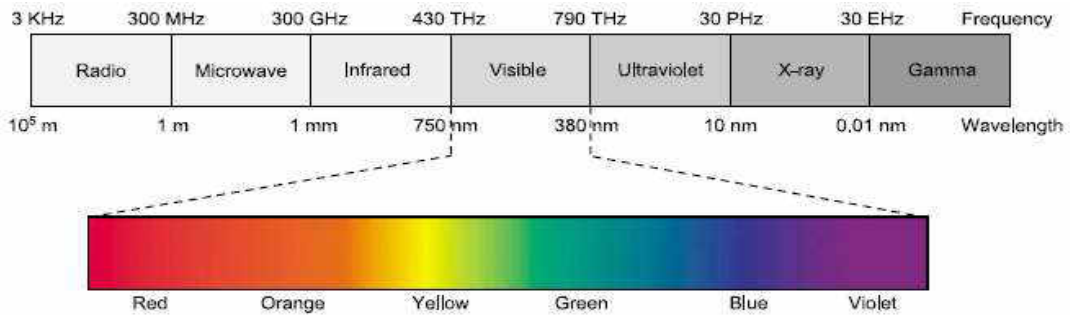
Figure 3. Human eye can perceive the electromagnetic signals between the frequency range of 430 THz and 790 THz which is referred as the visible light spectrum [7].
