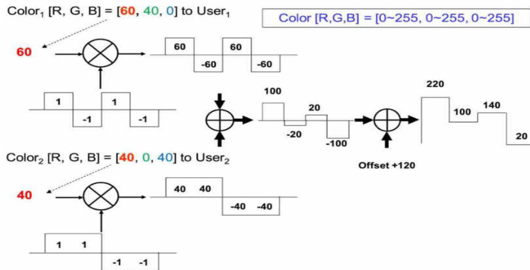
Figure 19. Tx of the proposed CSK-CDMA VLC system using red as an example.
