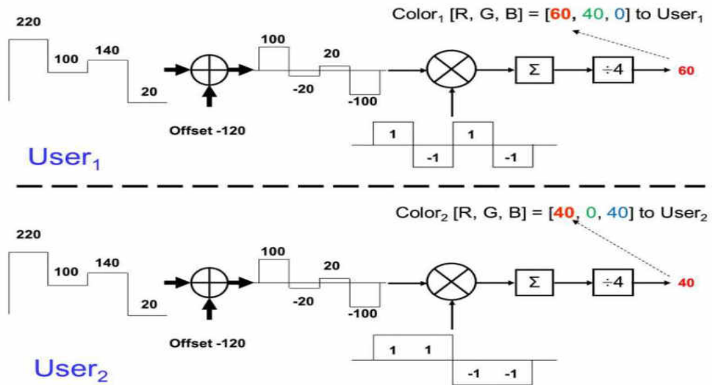
Figure 20. Rx of the proposed CSK-CDMA VLC system using red as an example.
