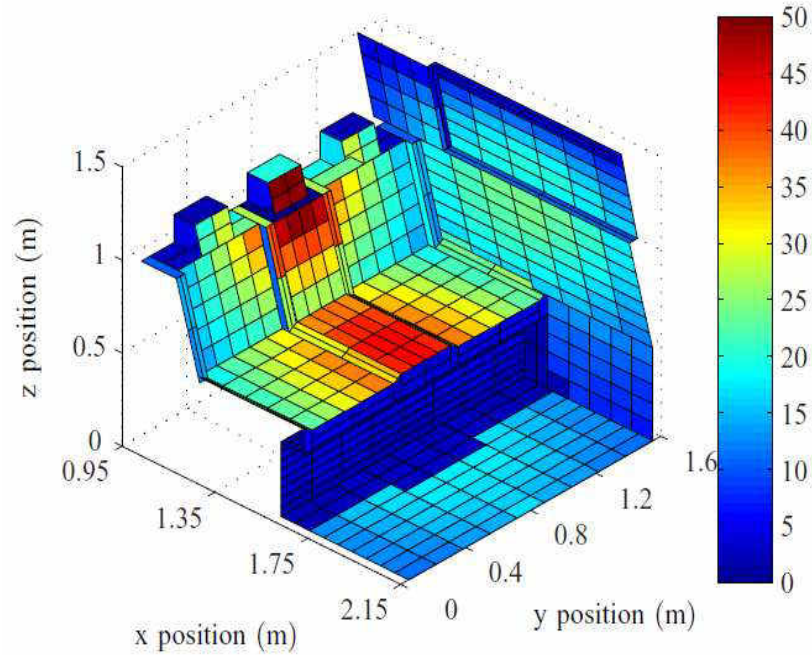
Figure 15. Received power in \mu\text{W} for the driver and front passenger seats[37].
