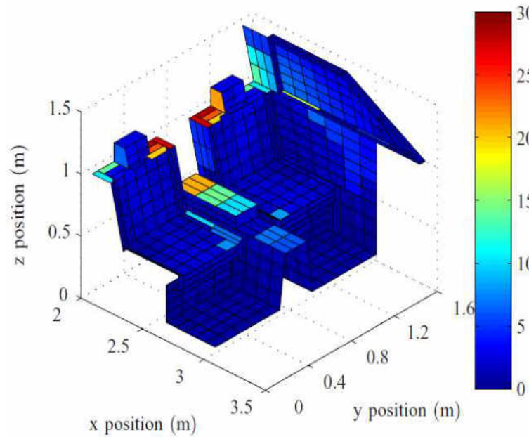
Figure 16. Received power in \mu\text{W} for the rear passenger seats [37].
