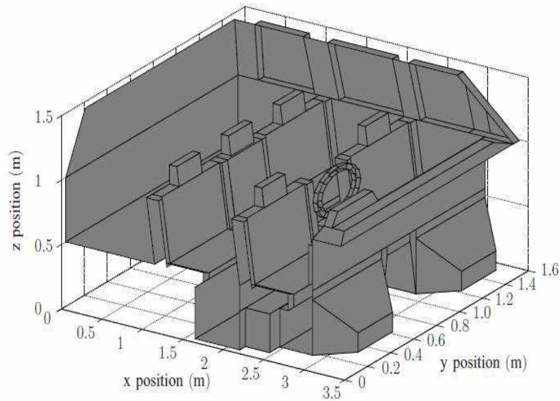
Figure 14. Front facing view of the deployment structure with the driver side wall, windscreen and ceiling removed [37].
