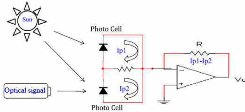
Figure 8. Differential optical receiver, illustrating sun light cancellation; I_{p1} and I_{p2} are photocurrents due to ambient light and optical signal, respectively[32].
