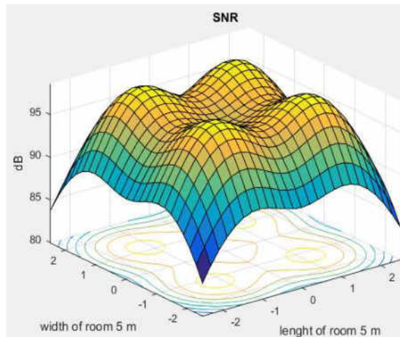
Figure 13. The SNR of receiver with optimization.
