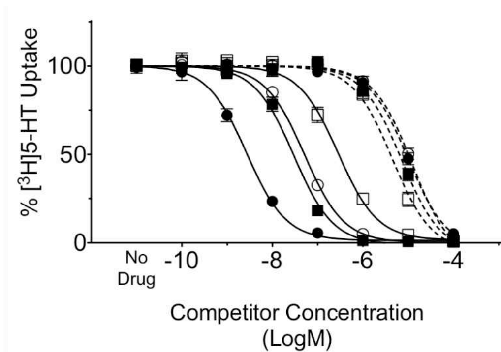
Figure 46. [^3\text{H}]5\text{-HT} uptake inhibition analysis for ( S )-citalopram, VK03-51, VK03-83 and NYDU-2-24. HEK-293 Griptide™ cells expressing hSERT (solid lines) or hSERT S438T (dashed lines) were assayed for [^3\text{H}]5\text{-HT} uptake in the presence of the indicated concentrations of ( S )-citalopram ( filled circles ), VK03-51 ( open squares ), VK03-83 ( open circles ) or NYDU-2-24 ( filled squares ). Data shown are means \pm SEM of transport activity for each form in the absence of competitor, set to 100%. Assays were conducted in triplicate and were repeated at least four times.
