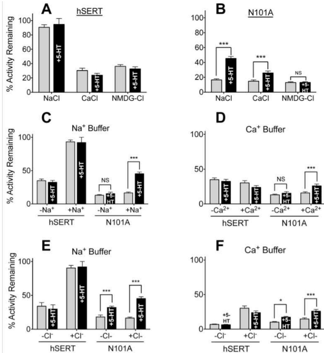
Figure 22. \text{Ca}^{2+} and \text{Na}^{+} alter C109 accessibility to MTSET, suggesting these cations may promote similar conformational changes in the N101A mutant. HEK-293 cells expressing hSERT or hSERT N101A were pretreated with 1mM MTSET in the absence ( gray bars ) or presence ( black bars ) of 5-HT (20 \mu\text{M} ) and in the presence of \text{Na}^{+} , \text{Ca}^{2+} or \text{NMDG}^{+} . Following treatment, 5-HT uptake assays were performed in complete buffer to quantitate activity. Percent remaining activity is plotted and is defined as the amount of 5-HT uptake of MTSET-treated cells as a percent of untreated cells. Each bar represents the mean and SEM of at least three independent experiments, each of which was performed in quadruplicate. Panels (A) & (B) depict results of MTSET treatment on (A) WT hSERT and (B) hSERT N101A in each cation buffer. Panels (C) and (D) represent data from (A) and (B) replotted with respect to genetic background and the presence or absence of \text{Na}^{+} (C) or \text{Ca}^{2+} (D). Panels (E) and (F) highlight the effect of \text{Cl}^{-} replacement under full \text{Na}^{+} (E) or full \text{Ca}^{2+} (F) buffer conditions. A two-tailed t -test was performed on sample sets as indicated with brackets; *** = p < 0.001 ; * = p < 0.05 ; n.s = not significant.
