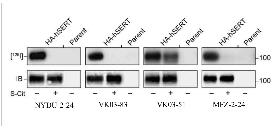
Figure 47. Photoaffinity labeling of hSERT. HA-hSERT LLCPK 1 cells or nontransfected (parent) LLCPK 1 cells were incubated with the indicated ligands in the absence (-) or presence (+) of 10μM ( S )-citalopram ( S-Cit ). Cell lysates were immunoprecipitated with Anti-HA antibodies followed by SDS-PAGE and autoradiography to detect [ 125 I] radiolabeled proteins ( upper panels ) or were analyzed by immunoblotting ( IB ) with anti-HA to detect total hSERT ( lower panels ). Results are representative of three independent experiments.
