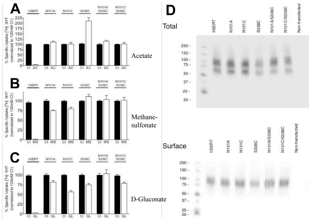
Figure 17. Anion replacement impact on 5-HT transport and substrate induced current in N101 and S336 mutants. [^3\text{H}]5\text{-HT} (30 nM) uptake in HeLa cells was determined under \text{Cl}^- -replacement with the anions (A) acetate, (B) methanesulfonate and (C) D-gluconate in hSERT and mutants as marked. Data were normalized to uptake of \text{Cl}^- -containing buffer for each mutant. (D) Western blot analysis was conducted to determine the surface expression of each hSERT mutant. Surface proteins were labeled with a biotin tag, purified using neutravidin beads. hSERT was detected using the monoclonal antibody ST51-1. Parental cells are included as a control.
