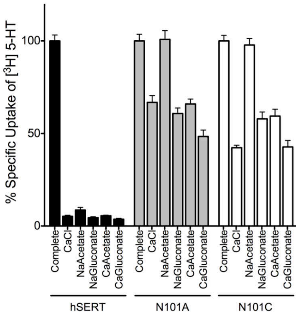
Figure 21. 5-HT uptake in N101 mutants under cation and/or anion ion replacement. Transport activity was measured in HEK cells stably expressing hSERT, N101A or N101C. Initial transport rates (10 min.) were obtained in complete buffer or in the presence of a buffer in which NaCl is replaced with 60mM CaCl 2 , 120mM Na-acetate, 60mM Ca-acetate or 60mM Ca-gluconate. Activity was normalized to activity in complete buffer. Each bar represents the mean and SEM of three separate experiments, each performed in quadruplicate. Data were analyzed using a two-way ANOVA and Bonferroni post-hoc test.
