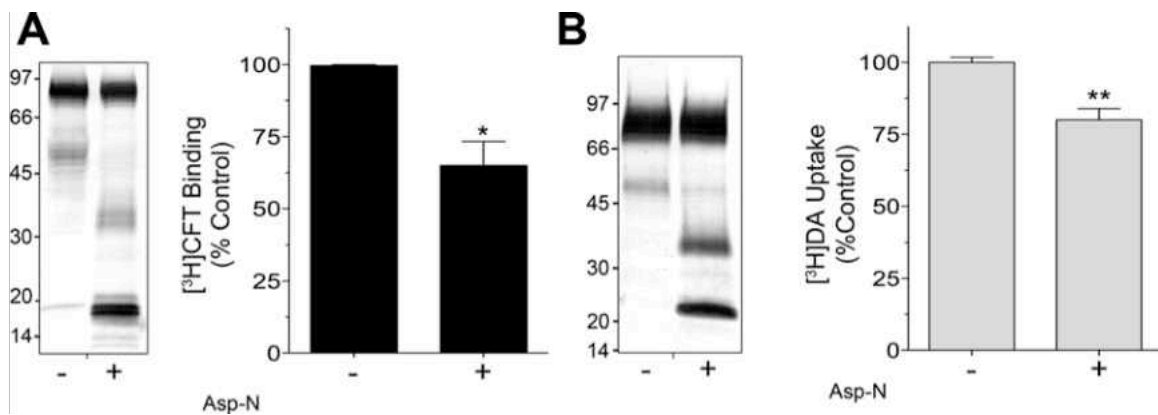
Figure 34. Asp-N treatment disrupts binding and transport activities. (A) Rat striatal membranes or (B) rat striatal synaptosomes were treated with (+) or without (-) 5 \mu g/ml Asp-N followed by assessment of (A) [ 3 H]CFT binding or (B) [ 3 H]DA uptake. Left panels show verification of proteolysis by immunoblotting. Histograms show quantification of uptake or binding ( means \pm S.E.M. ). * = p < 0.05 , ** = p < 0.01 relative to control by Student's t-test.
