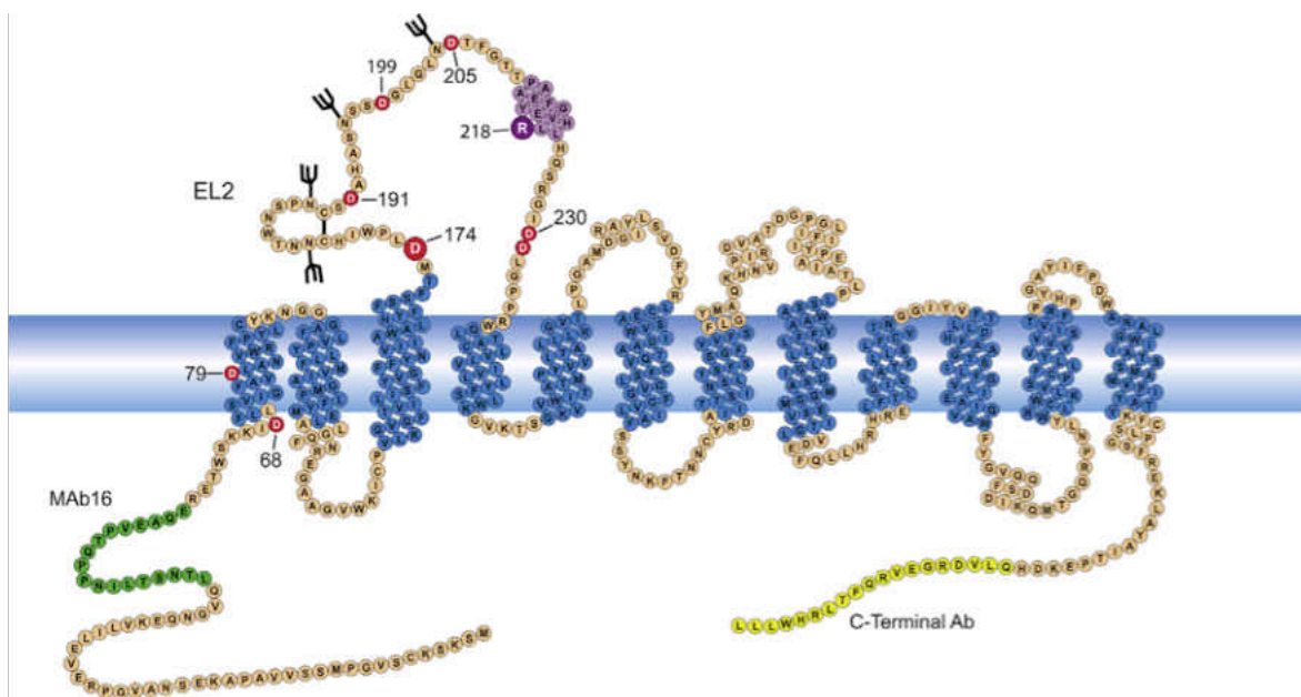
Figure 30. Two-dimensional diagram of DAT. (A) Schematic diagram of rDAT illustrating 12 transmembrane spanning domains, epitopes for N- and C-terminal tail antibodies ( green and yellow ), and EL2 components including N-linked glycosylation ( branched structures ), disulfide bond ( solid line ), Asp residues ( red circles ), D174 ( large red circle ) and R218 ( large purple circle ). The full rDAT sequence was analyzed by PsiPred and JUFO secondary structure prediction algorithms, which predicted the region surrounding and including R218 is likely a helical structure ( purple ).
