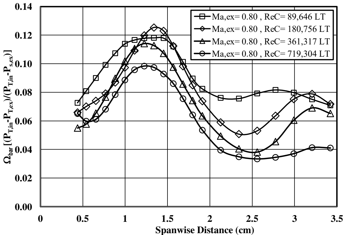
Figure 51. Cross-passage averaged total pressure loss coefficient \Omega (Omega) for the vane at \frac{1}{4} axial chord location under low turbulence over a range of Reynolds numbers of 90,000, 180,000, 360,000, and 720,000 at a Mach number of 0.8.
