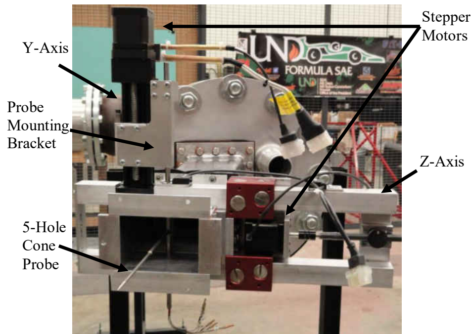
Figure 15. The five-hole cone probe traversing system used for exit velocity surveys during aerodynamic secondary loss testing.
