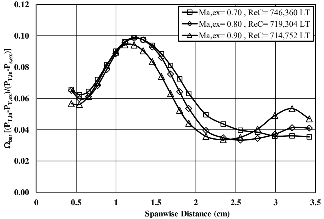
Figure 62. Cross-passage averaged total pressure loss coefficient \Omega (Omega) for the vane at \frac{1}{4} axial chord location under low turbulence over a range of Mach numbers of 0.7, 0.8, and 0.9 at a Reynolds number of 720,000.
