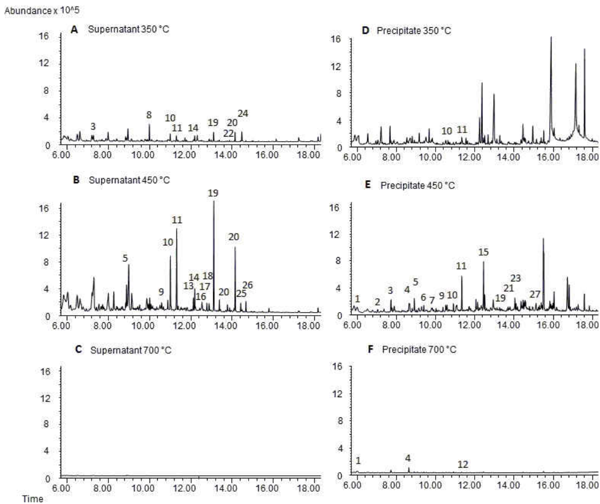
Figure 4. TD-Pyr-GC-MS chromatograms showing the distribution of methoxyphenols and aromatics (for labels of identified chemicals see Table 3) for biodecomposition with combination of C. versicolor and T. gallica after 57 days. Panels A (350 °C), B (450 °C), C (700 °C) represent the composition of the supernatant (decanted solution) after 57 days of incubation (as detailed in Section 3.6). Panels D (350 °C), E (450 °C), F (700 °C) reflect the composition of the precipitate in the same sample (57 days).
