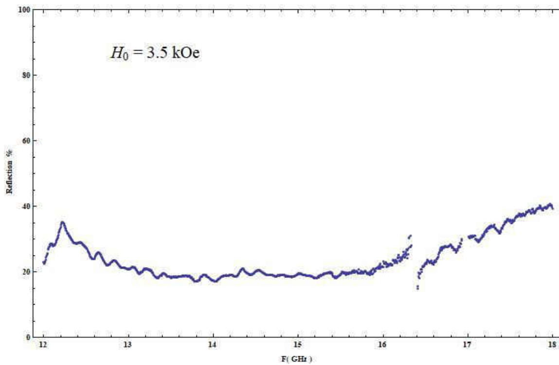
Fig. 4.7. 65 Reflection vs. Frequency for H_0 = 3.5 kOe
