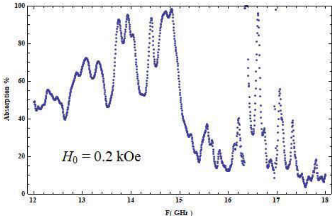
Fig. 4.7.12 Absorption vs. Frequency for H_0 = 0.2 \text{ kOe}
