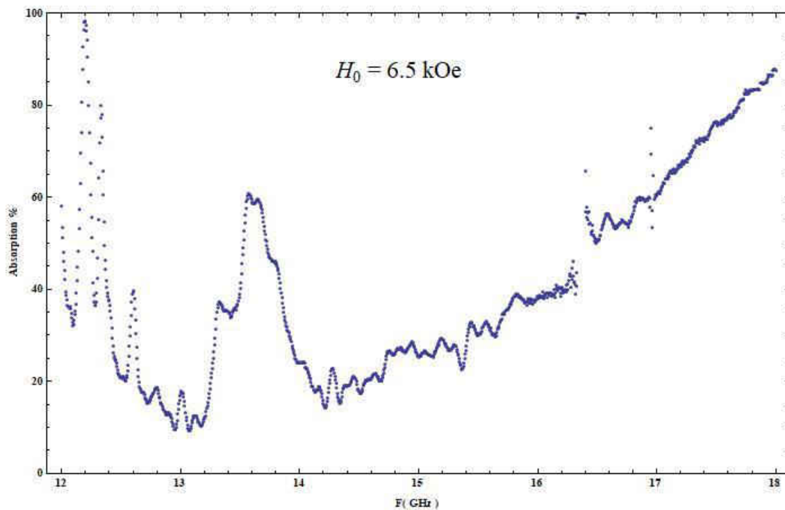
Fig. 4.7.78 Absorption vs. Frequency for H_0 = 6.5 \text{ kOe}
