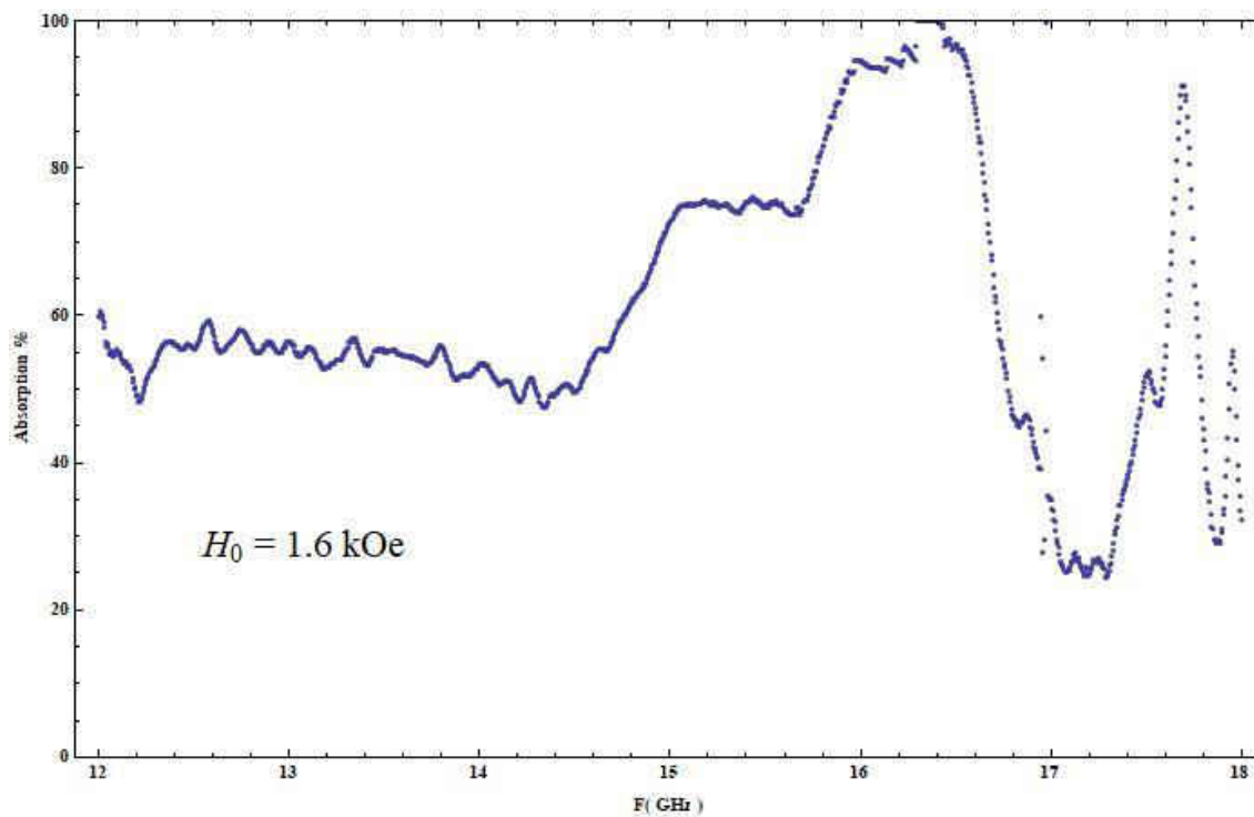
Fig. 4.7.51 Absorption vs. Frequency for H_0 = 1.6 kOe
