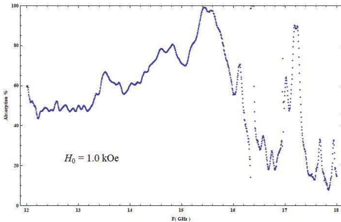
Fig. 4.7.39 Absorption vs. Frequency for H_0 = 1.0 kOe
