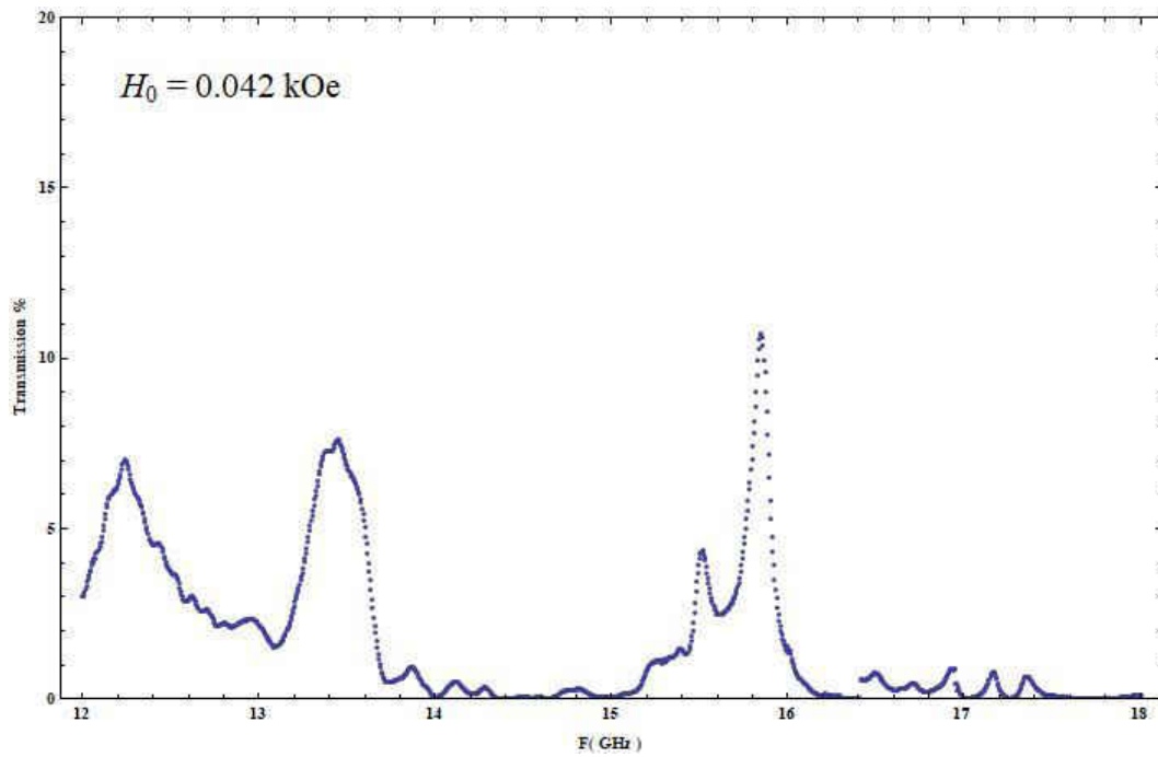
Fig. 4.7.1 Transmission vs. Frequency for H_0 = 0.042 kOe
