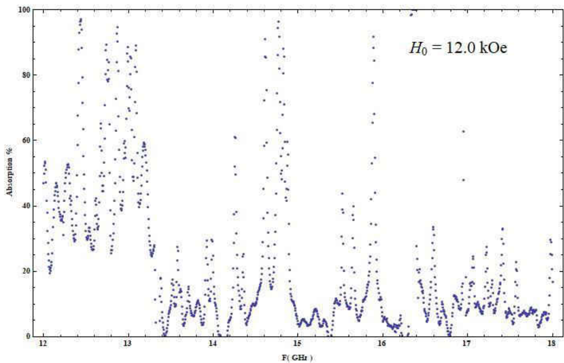
Fig. 4.7.111 Absorption vs. Frequency for H_0 = 12.0 \text{ kOe}
