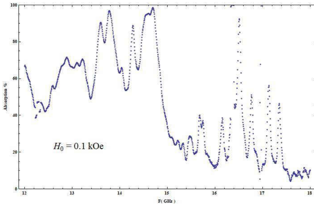
Fig. 4.7.6 Absorption vs. Frequency for H_0 = 0.1 \text{ kOe}
