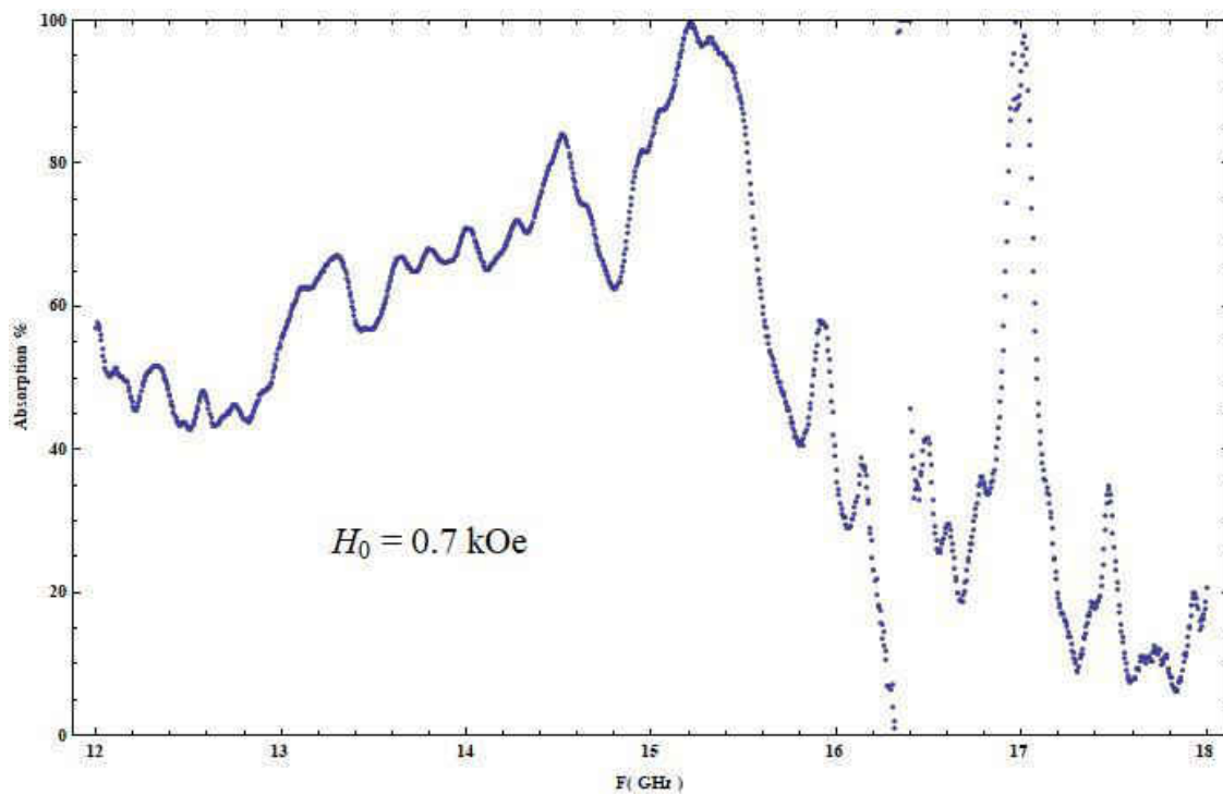
Fig. 4.7.30 Absorption vs. Frequency for H_0 = 0.7 kOe
