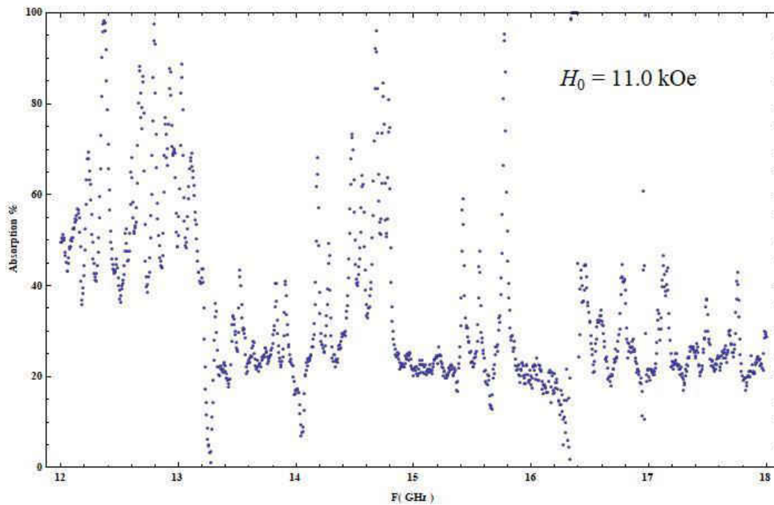
Fig. 4.7.105 Absorption vs. Frequency for H_0 = 11.0 kOe
