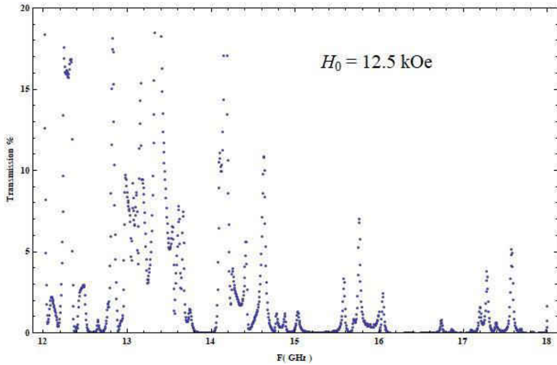
Fig. 4.7.112 Transmission vs. Frequency for H_0 = 12.5 \text{ kOe}
