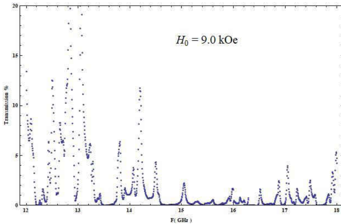
Fig. 4.7.91 Transmission vs. Frequency for H_0 = 9.0 \text{ kOe}
