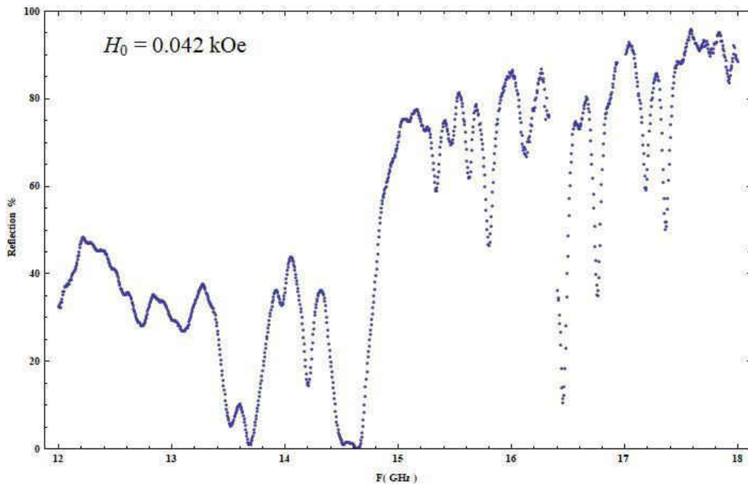
Fig. 4.7.2 Reflection vs. Frequency for H_0 = 0.042 kOe
