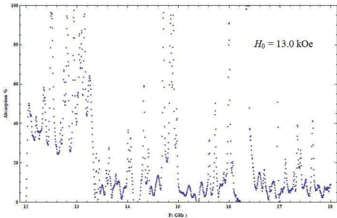
Fig. 4.7.117 Absorption vs. Frequency for H_0 = 13.0 kOe
