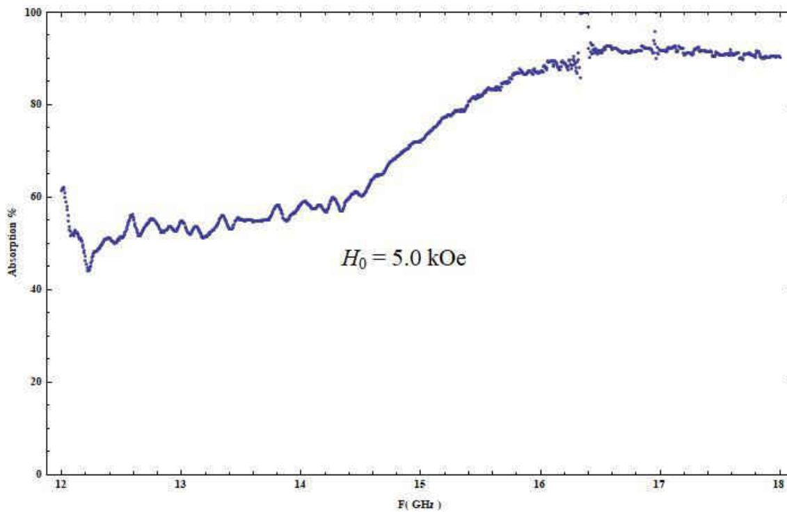
Fig. 4.7.72 Absorption vs. Frequency for H_0 = 5.0 kOe
