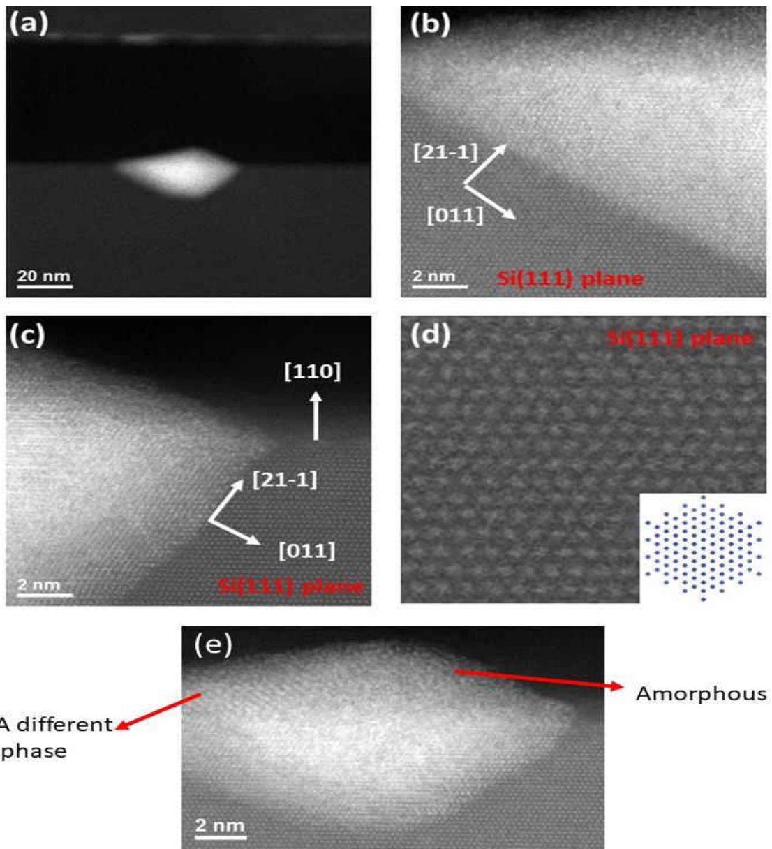
Figure 5.2. (a) shows a cross-sectional image of a NW grown under similar conditions. (b) and (c) are higher resolution images of the same NW. (d) shows a higher resolution image of the Si (111). Inset: is a model of the bulk Si oriented towards (111) direction. (e) Shows a cross-section of another nanowires top-left part of the nanowire has another phase and the rest of the top part looks amorphous.
