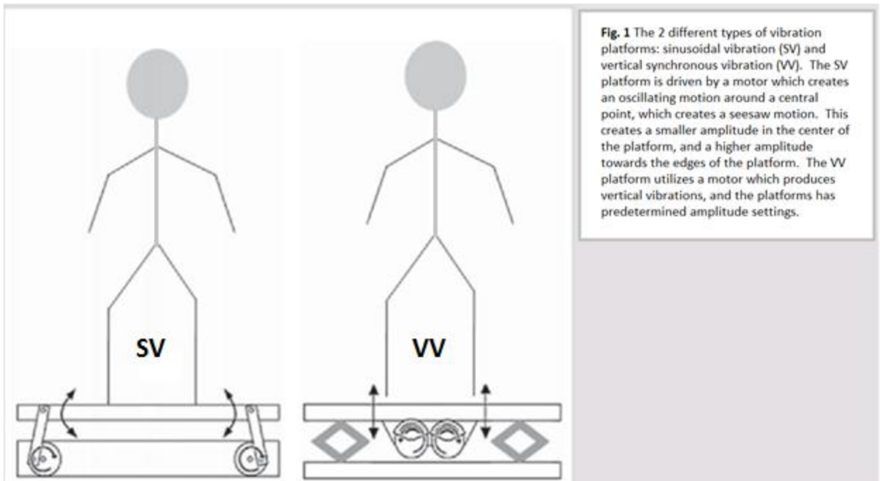
Figure 1: Vibration Platform Design Comparison: Sinusoidal and Vertical Vibration
