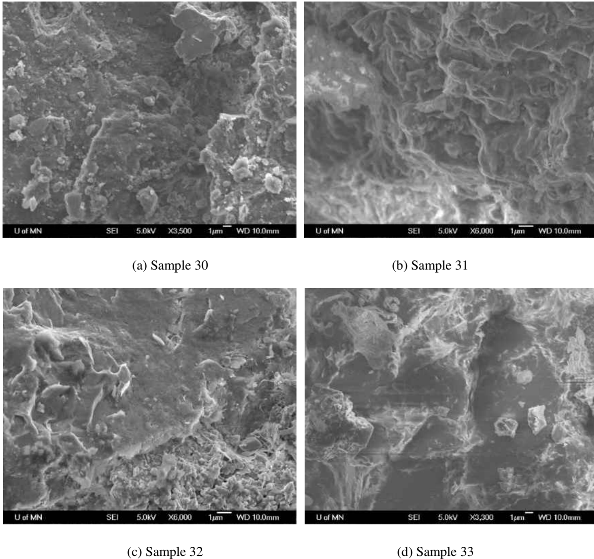
Fig. 6.12. SEM images of few shale samples from different members of the Bakken Formation.
