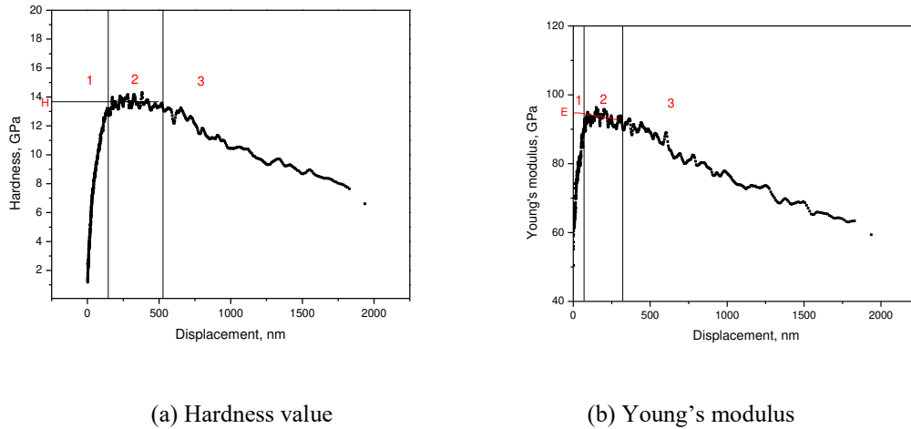
Fig. 6.8. Changes of elastic modulus and Hardness versus penetration depth. Both plots show three distinguished stages: 1. Initial rising; 2. Plateau; 3. falling off.
