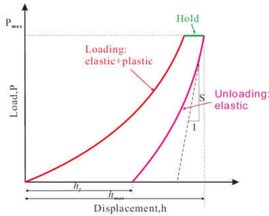
Fig. 6.1. Schematic illustration of indentation load–displacement curve (Hu and Li, 2015).
