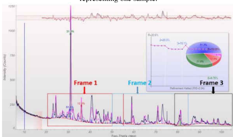
Fig. 6.10. Image of 3 Frames of 2D XRD scanning for angles of (a) of 25-55°, (b) 55-85° and (c) 85-115° representing one sample.
