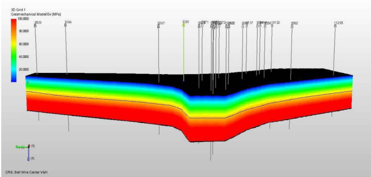
Fig (38). View of Blue Buttes grid populated with Overburden Stress.
