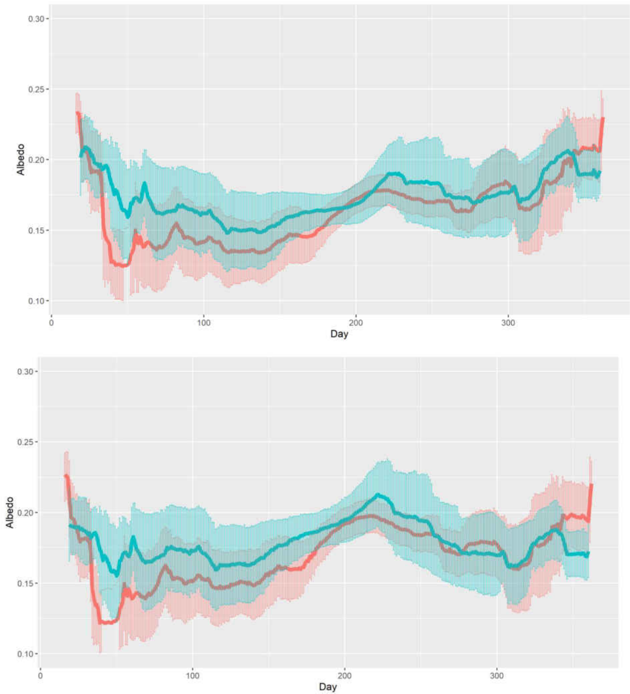
Figure 21: (a) Total shortwave, black-sky albedo by Julian day of maize (red) and spring wheat (blue) in HZ4. (b) Total shortwave, white-sky albedo by Julian day of maize (red) and spring wheat (blue) in HZ4.
