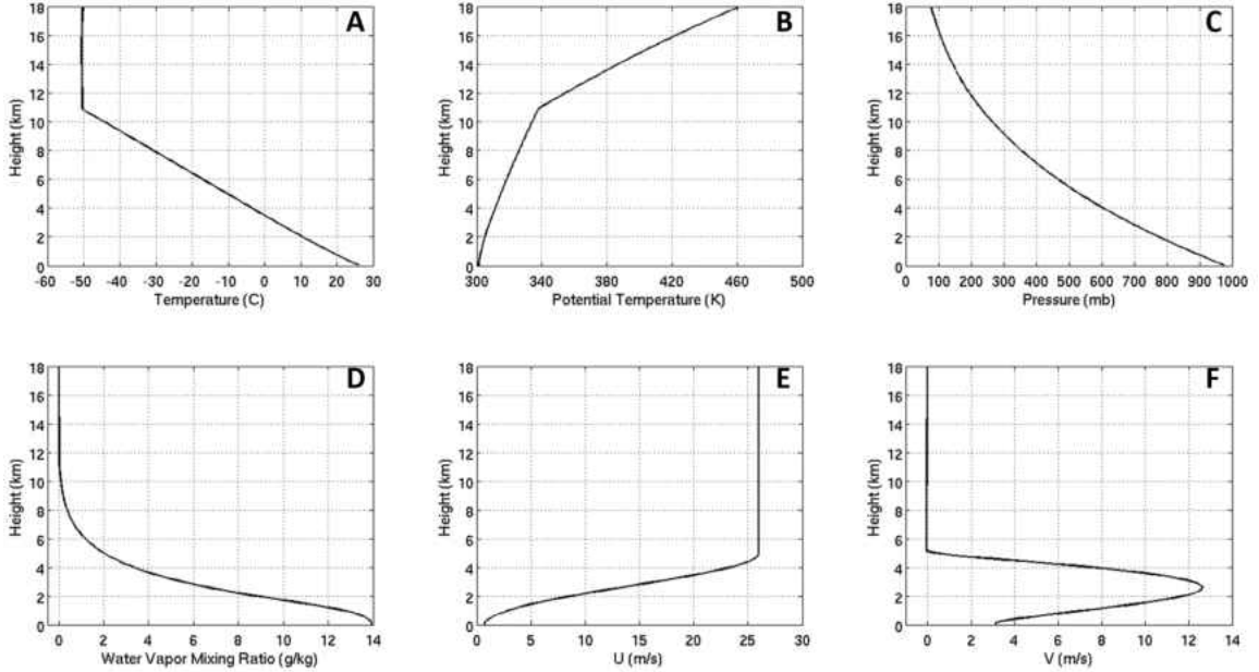
Figure 3: The initial profiles for the input sounding are shown. Plot A shows the initial temperature profile, B shows the potential temperature profile, C shows the pressure profile, D shows the water vapor mixing ratio in the moist section of the domain, E the u-winds, and F shows the v-winds.
