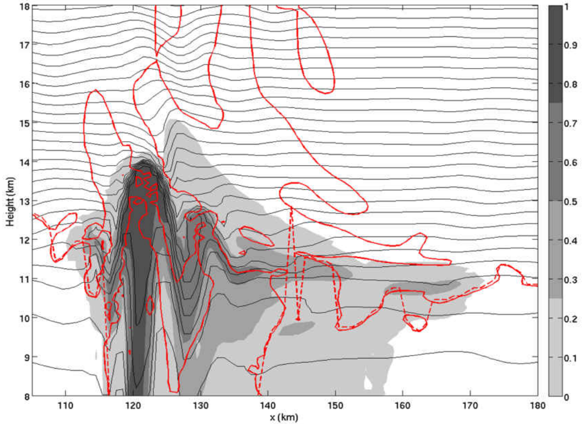
Figure 14: Vertical cross section through the maximum updraft at 1 hour, focusing on 8 km – 18 km. Grayscale contours are boundary layer tracer in \text{kg kg}^{-1} . The minimum boundary layer concentration depicted is 0.001 \text{ kg kg}^{-1} . Thin black lines are isentropes from 295 K to 500 K with a contour interval of 5 K, solid red line is the contour of PV, dashed red line is the first altitude at which the PV threshold was met. It should be noted that the tropopause is restricted to be only above 8 km.
