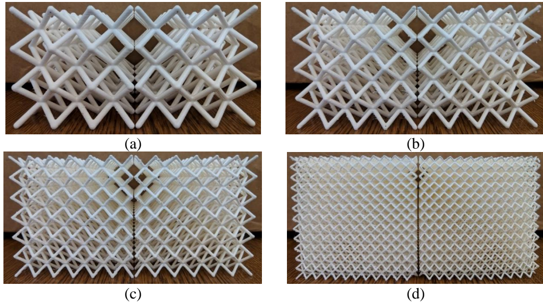
Figure 1: Pictures of one full replication with 8 specimens, with as-built (left) and acetone-smoothed (right) specimens of cell size (a) 25.40mm (1.00 in), (b) 19.05 mm (0.75 in), (c) 12.70 mm (0.50 in), and (d) 6.35 mm (0.25 in)
