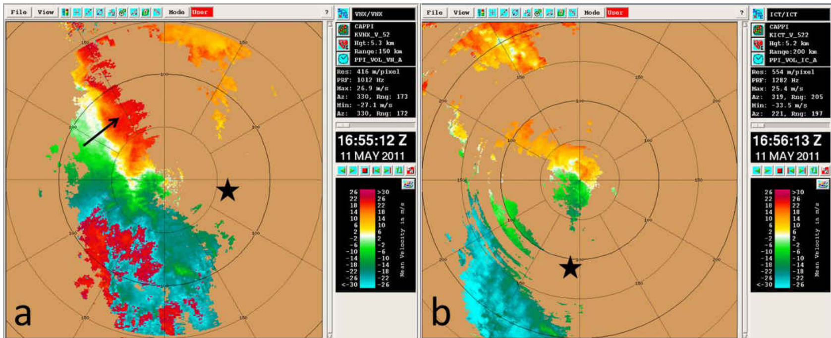
Figure 23: Radial velocity CAPPIS at 5.6 km MSL from (a) Vance Air Force Base, Oklahoma (KVNIX) radar on 11 May 2011 at 16:55 UTC and (b) Wichita, Kansas (KICT) radar at 16:56 UTC. Arrow indicates wind direction across the zero isodop.
