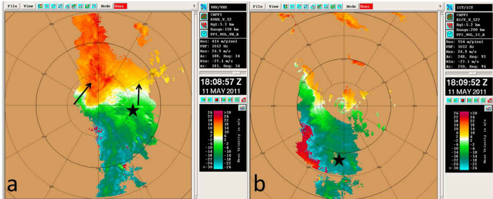
Figure 26: Radial velocity CAPPIs at 5.6 km MSL from (a) Vance Air Force Base, Oklahoma (KVNIX) radar on 11 May 2011 at 18:09 UTC and (b) Wichita, Kansas (KICT) radar at 18:10 UTC. Arrows indicate wind direction across the zero isodop.
