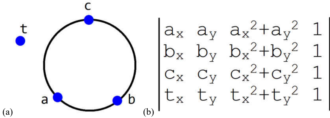
Fig. 11. (a) Two-dimensional in-circle test; (b) Matrix used to evaluate the two-dimensional in-circle test
