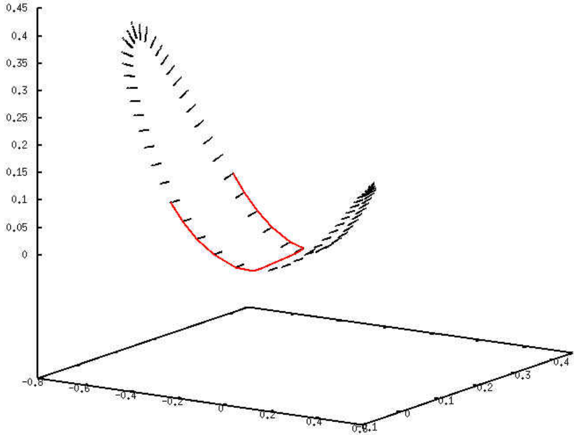
Fig. 19. NACA 0012 Airfoil with boundary layer vertices projected onto a paraboloid centered at the median vertex with dividing path (red)
