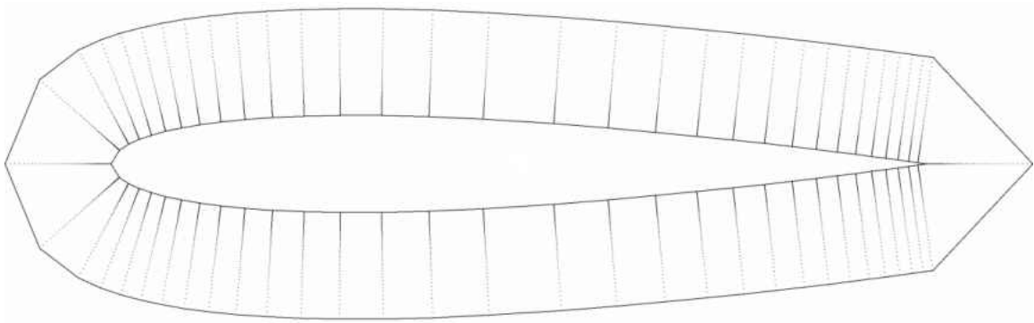
Fig. 8. NACA 0012 Airfoil with vertices inserted along surface normals
