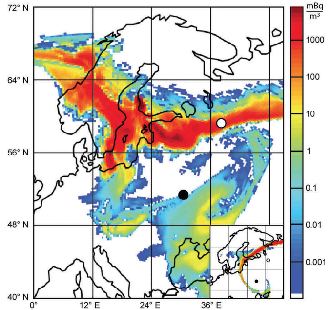
Fig. 5. A calculated surface air 133 Xe concentration map at 09:00 UTC on April 29 for one maximum power channel with a 75-ton explosion injecting its full debris into the 2.5- to 3.0-km altitude interval between 21:00 and 22:00 UTC on April 25, 1986. Note that “●” indicates the power plant and “○” marks Cherepovets. The inset in the lower right shows the cloud at the altitude of 3 km at midnight the day before the detection.
