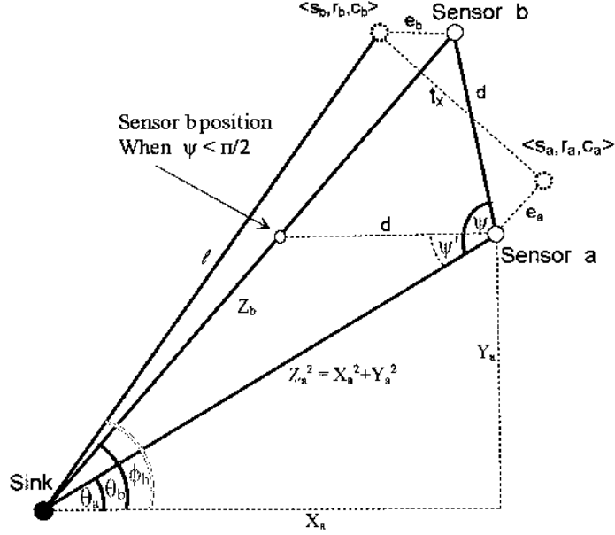
FIG. 7: Case 2: estimation of e_b^2
