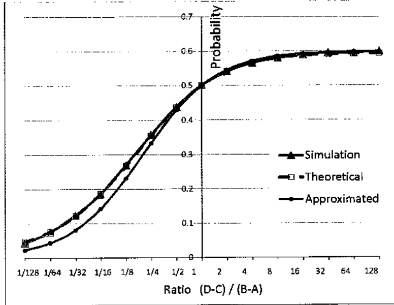
FIG. 36: Empirical validation of Theorem V.2.1
