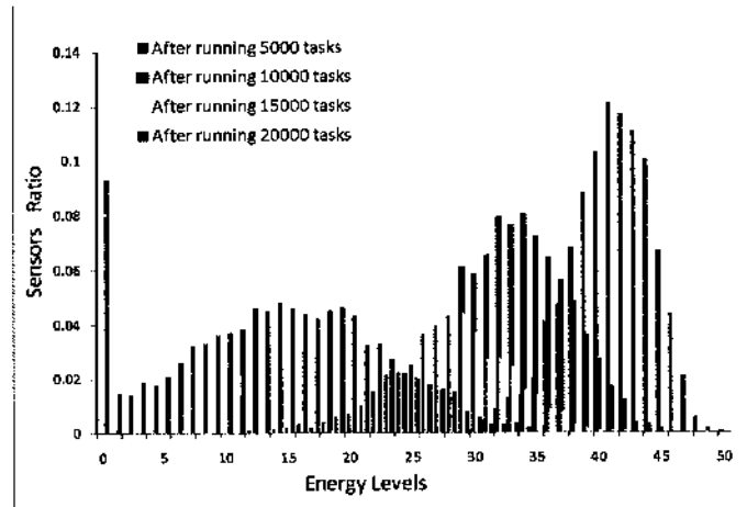
(a) Static Scheduling
