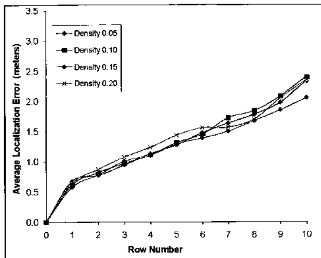
(a) Errors in distance measurements
