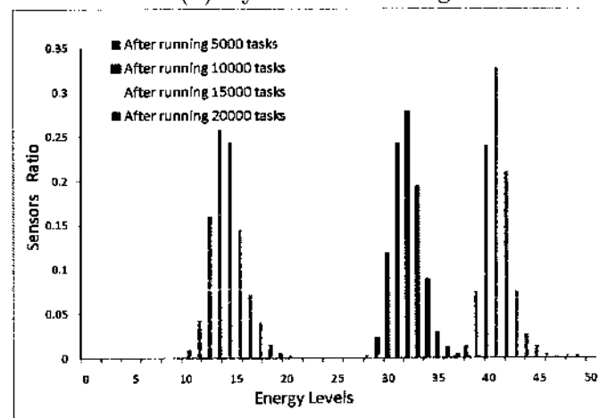
(c) Energy-Aware Scheduling
