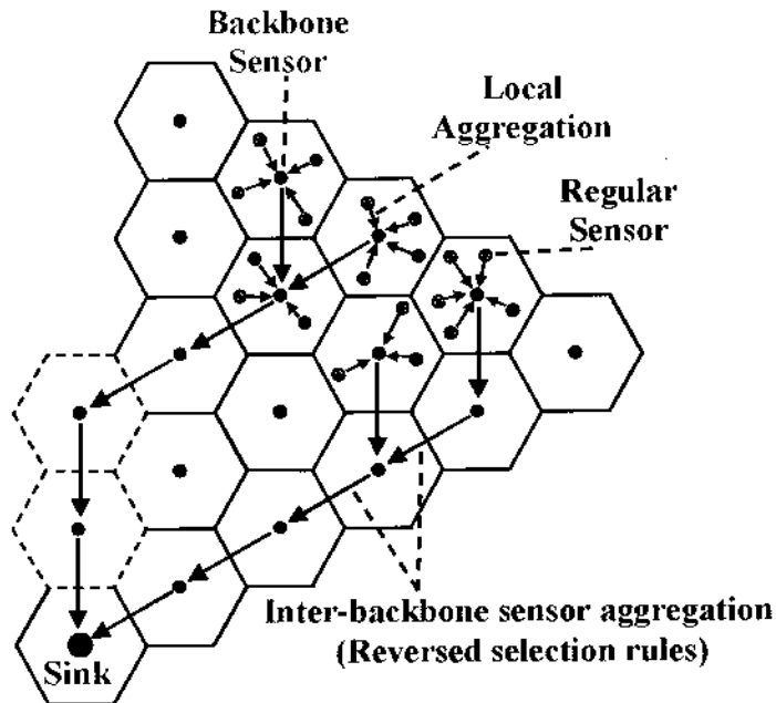
FIG. 14: Data aggregation and routing through our backbone
