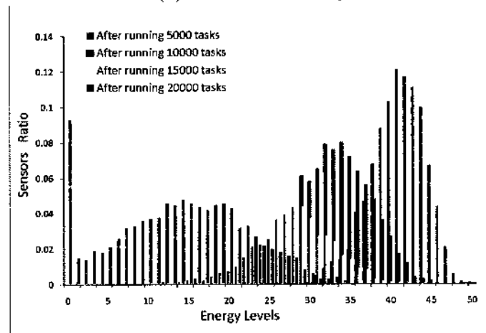
(b) Dynamic Scheduling
