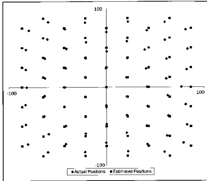
FIG. 17: Actual vs estimated positions of backbone sensors.
