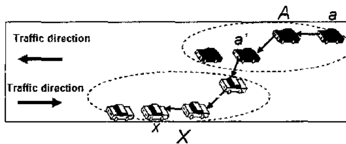
FIG. 29: OPERA: illustrating the Baseline Algorithm
