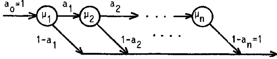
FIG. 38: Cox distribution
