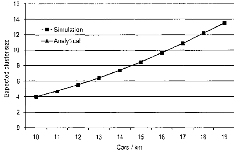
FIG. 22: Cluster size
