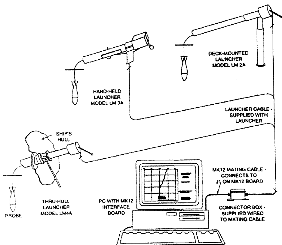
Fig. 42. Complete XBT Measurement System
