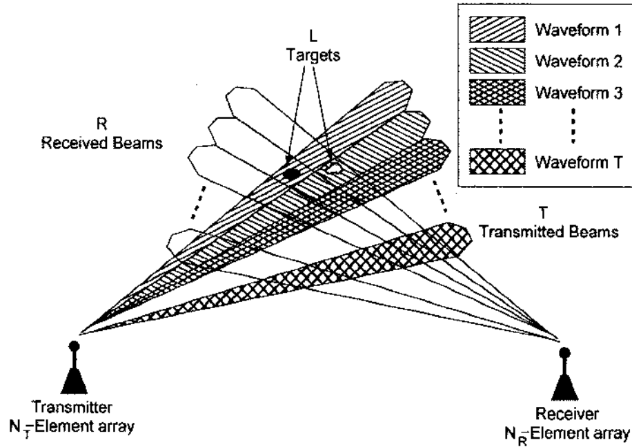
Fig. 3: System setup
