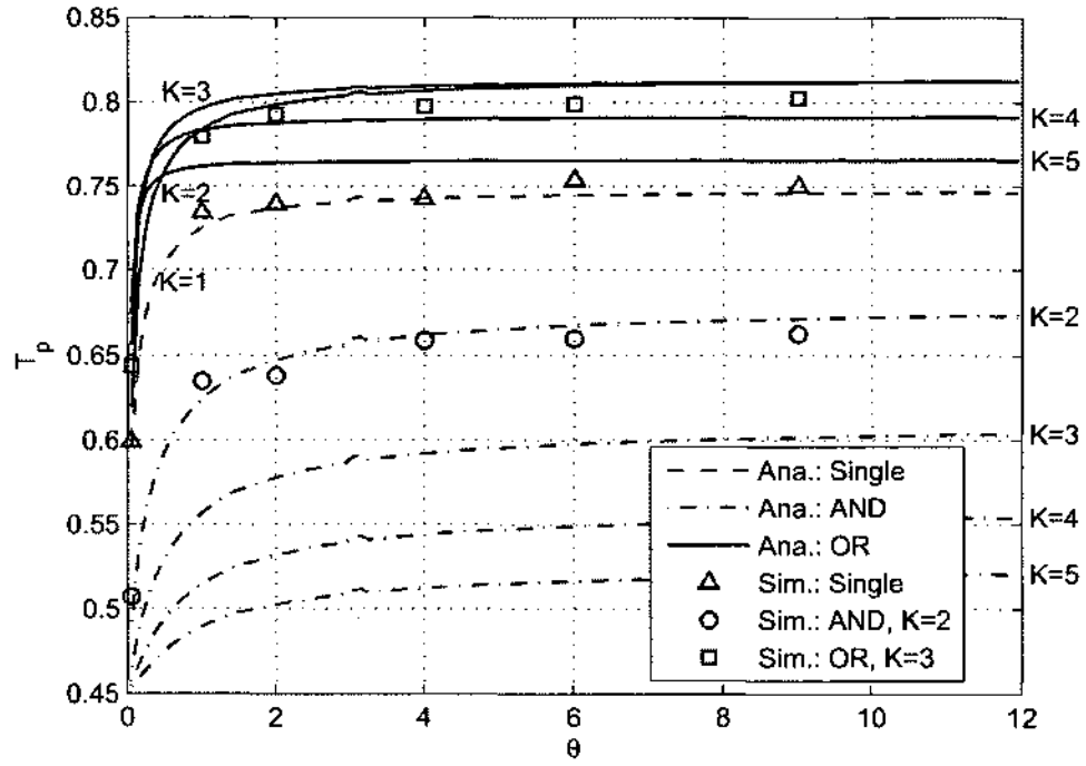
(a) The threshold \lambda is computed based on P_{f,d} = 0.1 .
