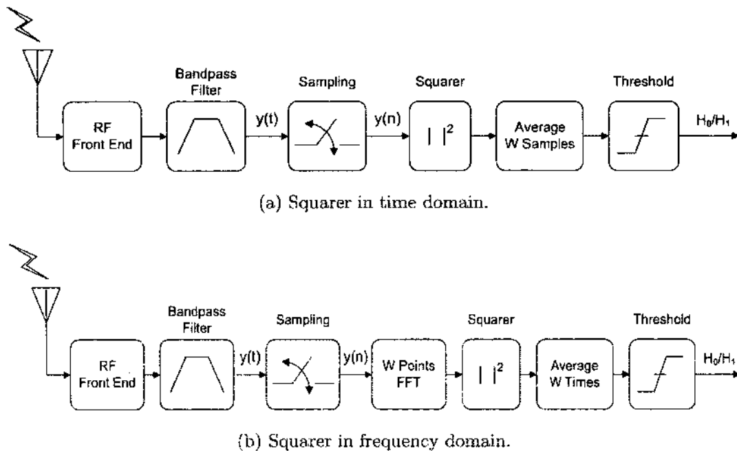
Fig. 2: Basic block diagrams of CR energy detector.
