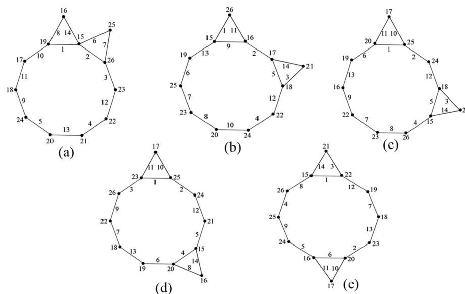
Figure 4. Labeling of non-isomorphic wounded flowers WF(10, 2) .
