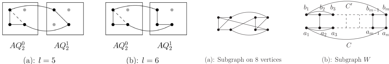
Figure 7. 3-regular subgraphs of AQ_n .
