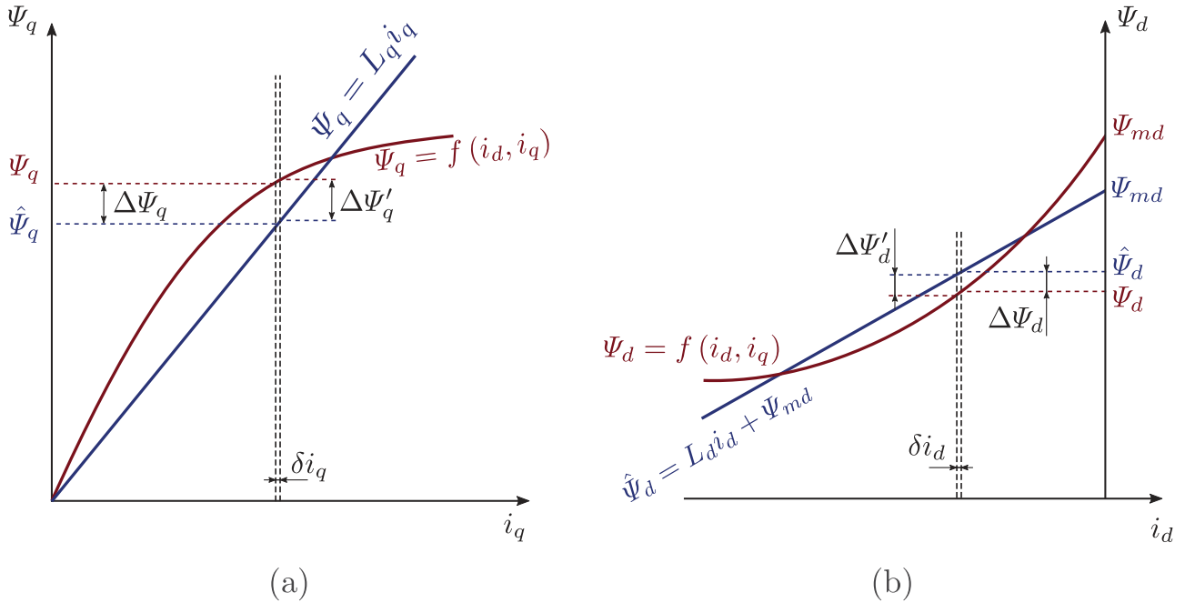
Figure 8. Flux as a function of current: (a) q axis and (b) d axis flux component.
