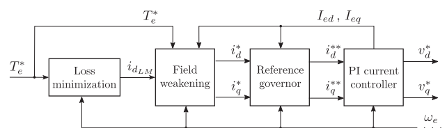
Figure 4. Field weakening and current reference governor position in control scheme.
