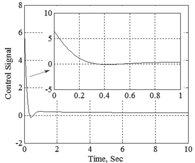
Figure 12. The control signal for Example 3.
