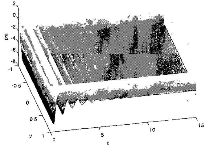
FIG. 57: Evolution of the peak alignment angle ( \phi ) across the entire plate gap for Er = 1000 , De = 12 , with parallel anchoring conditions at the plates ( \psi_o = 0^\circ ).
