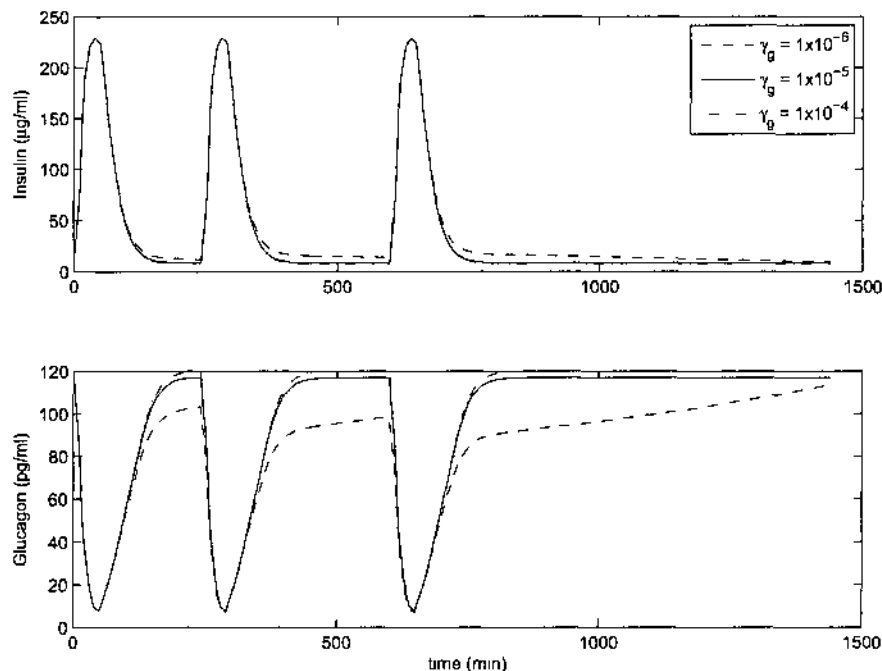
Fig. 10 Insulin (top) and glucagon (bottom) concentration for three values of \gamma_g .
