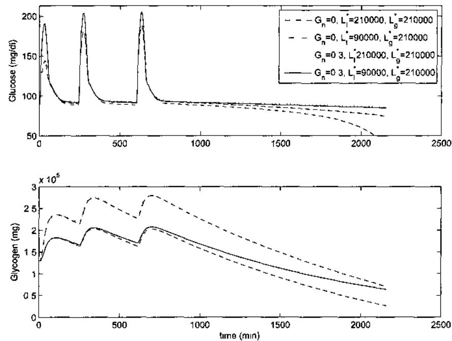
Fig. 20 Blood glucose concentration (top) and liver glycogen quantity (bottom) under gluconeogenesis with L_i^* \in \{90,000, 210,000\} mg, L_g^* = 210,000 mg, and G_n \in \{0, 0.30\} over a 36-hour time period.
