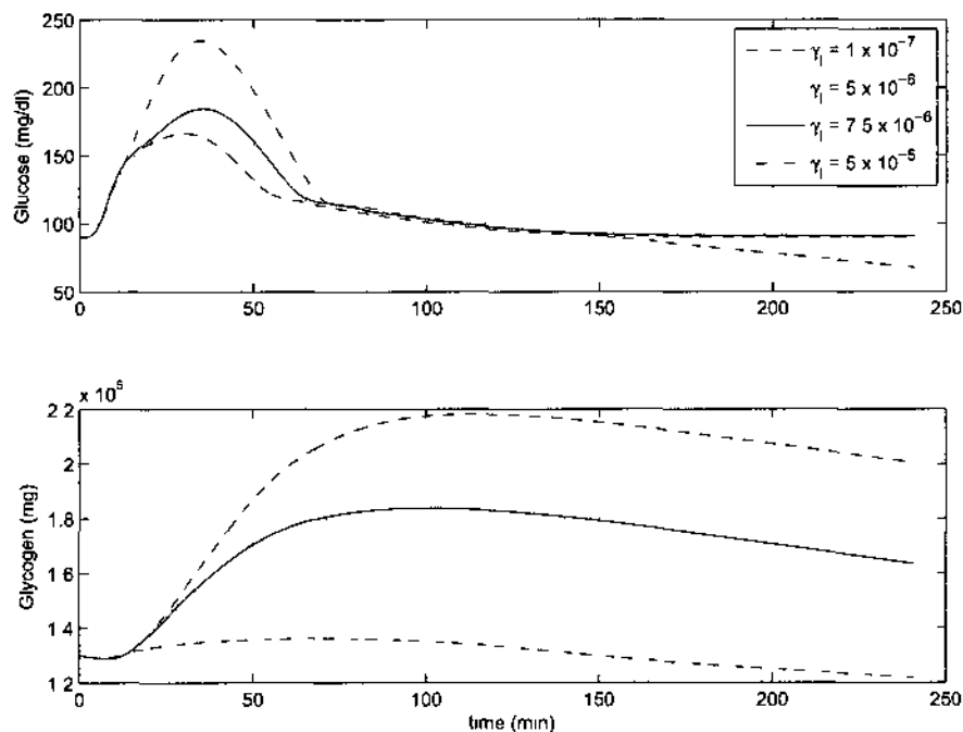
Fig. 5 Glucose concentration (top) and liver glycogen quantity (bottom) for four values of \gamma_I during the first meal.
