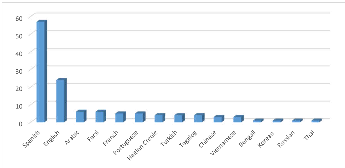
Figure 4. Language Distribution
