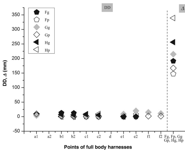
Figure 7. Strap slippage in adjustment buckles (DD) and dummy displacement \Delta in safety harness models F, G, and H. Note: a1, a2, b1, b2, c1, c2, d, e1, e2, f1, f2 = adjustment buckles/fitting on the harness; Fg, Gg, Hg = harness types equipped with a dorsal attachment point; Fp, Gp, Hp = harness types equipped with a sternal attachment point.
