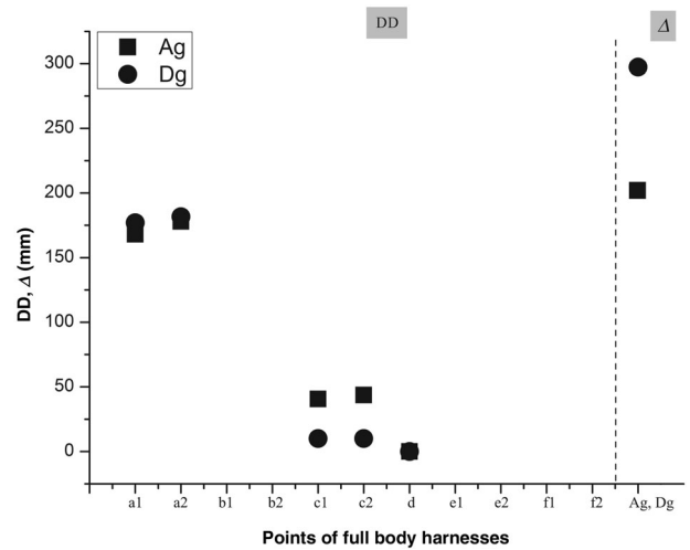
Figure 5. Strap slippage in adjustment buckles (DD) and dummy displacement \Delta in safety harness models A and D. Note: a1, a2, b1, b2, c1, c2, d, e1, e2, f1, f2 = adjustment buckles/ fittings on the harness; Ag, Dg = harness types equipped with a dorsal attachment point.
