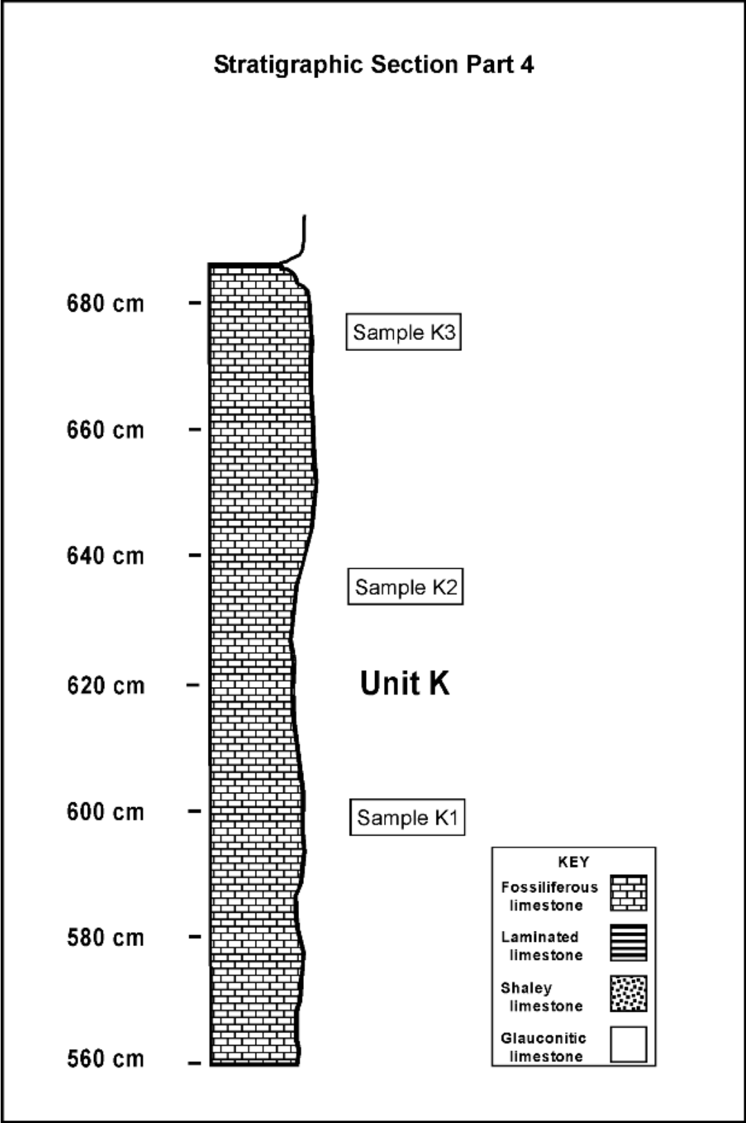
Figure 11. Stratigraphic section, part 4.
