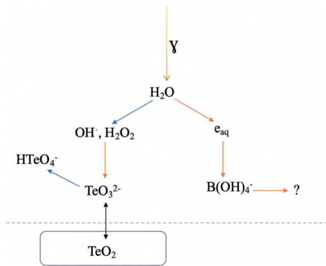
Fig. 6. Schematic presentation of the system with the TeO 2 precursor in ABS without the sodium thiosulfate additive.
