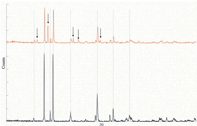
Fig. 5. XRD from (bottom line) nonirradiated TeO 2 and (top line) solid TeO 2 after 1.2 MGy irradiation in ABS with the sodium thiosulfate additive. Arrows point to the differences in the diffractograms identified as elemental tellurium. The coinciding TeO 2 peaks are marked with lines.
