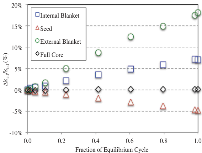
Fig. 12. Reactivity changes of seed, internal blanket, external blanket, and full core in “Large-Size” case.
