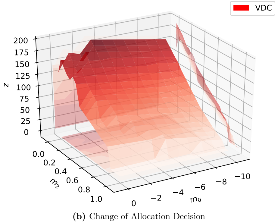
Figure 2.11: Value of Discrete Choice Model of Data Set: K = 4 , L = 7 , J = 3
