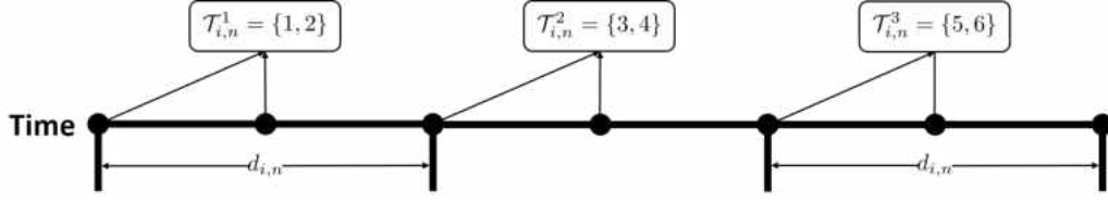
Figure 4.4: Partition of Time Set
