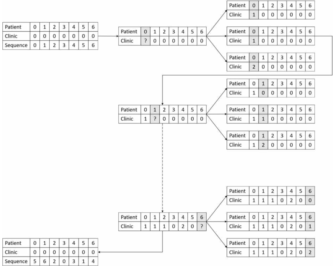
Figure 2.6: GA-GLS: Iteration update
