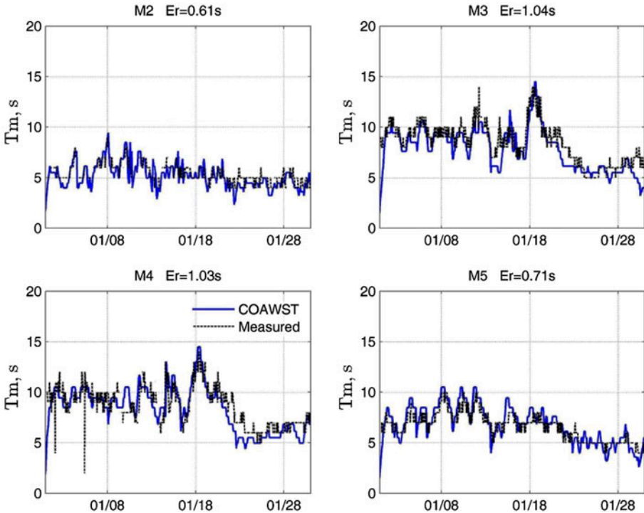
Figure 8. Validation of the COAWST wave period results at a number of wave buoys (table 3) during January 2005.
